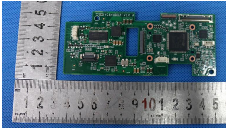
Photo-06 Component view of VC84UDDA board
