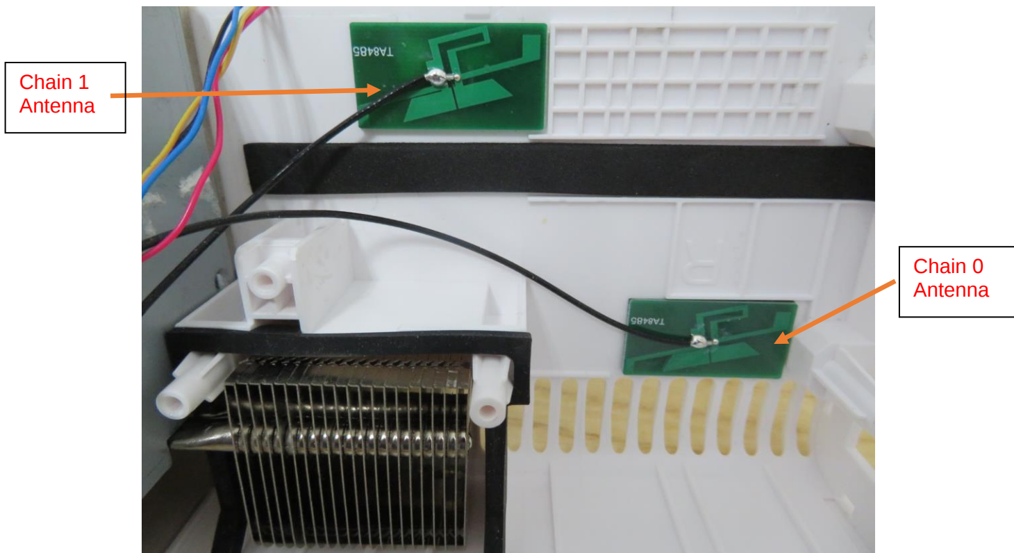
Photo-15 Wireless module
