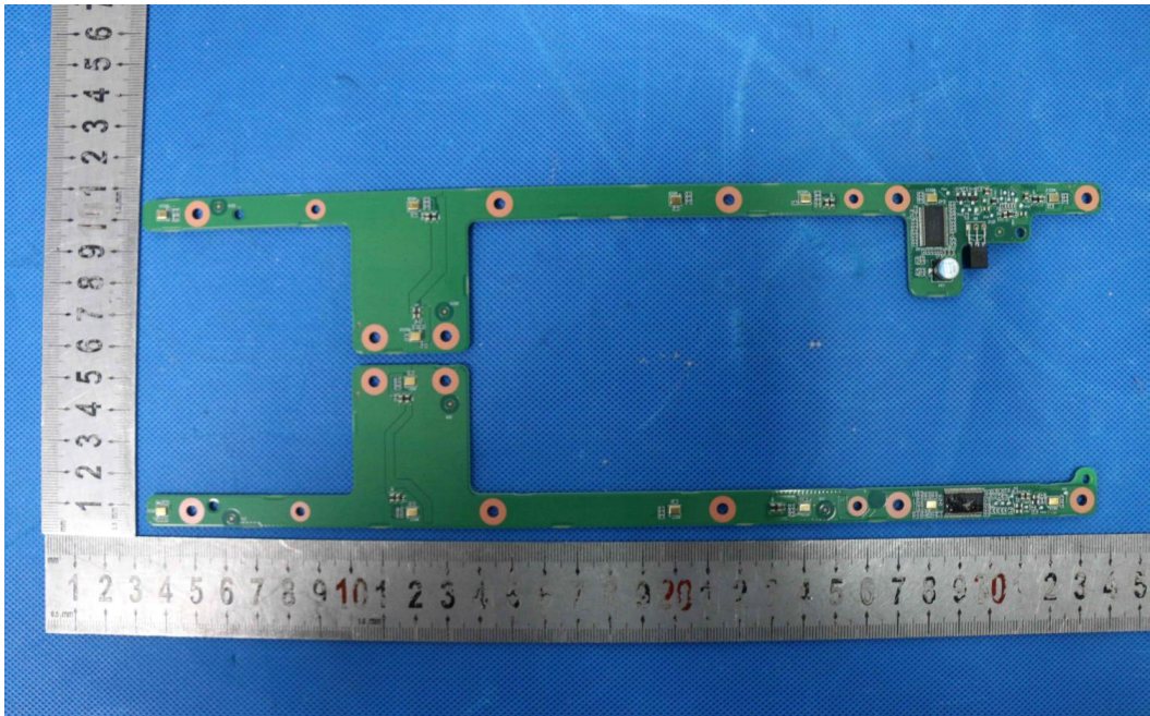
Photo-13 Component view of VC84UDBA board
