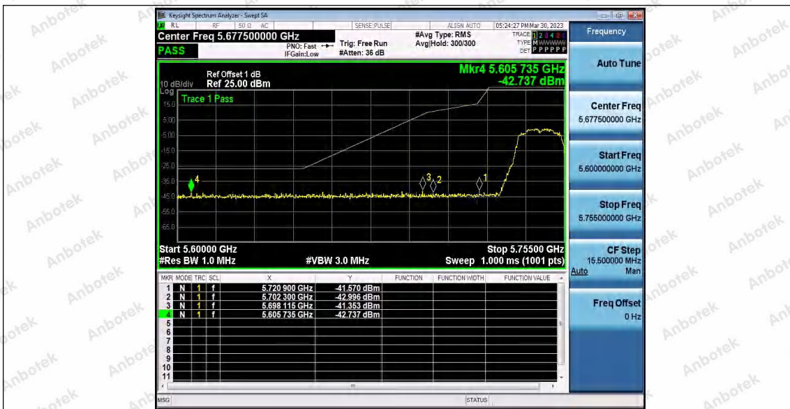
11AC20SISO_Ant2_Low_5745
