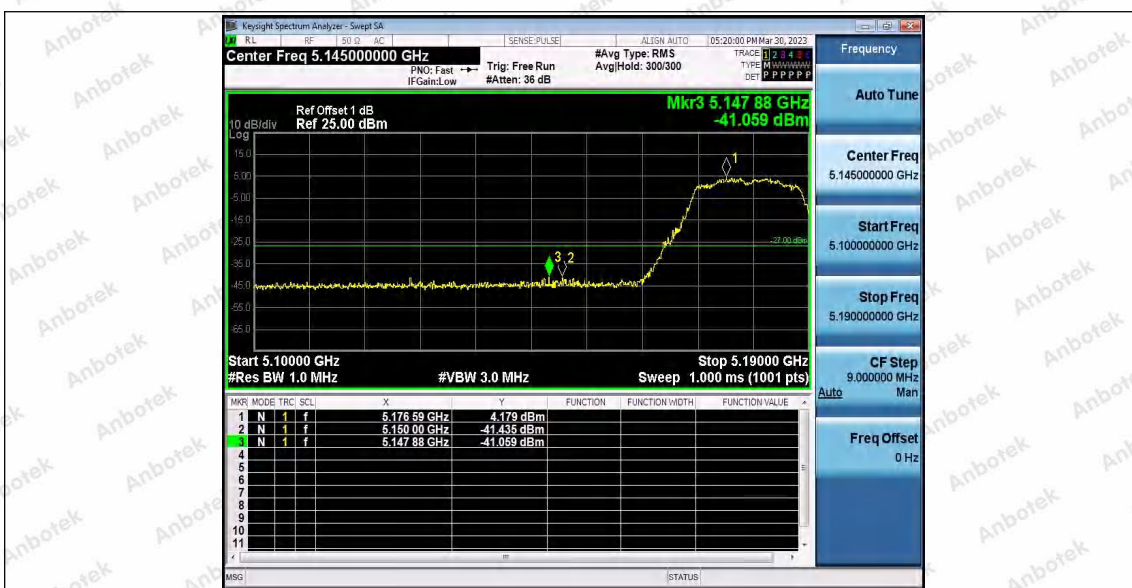
11AC20SISO_Ant2_Low_5180
