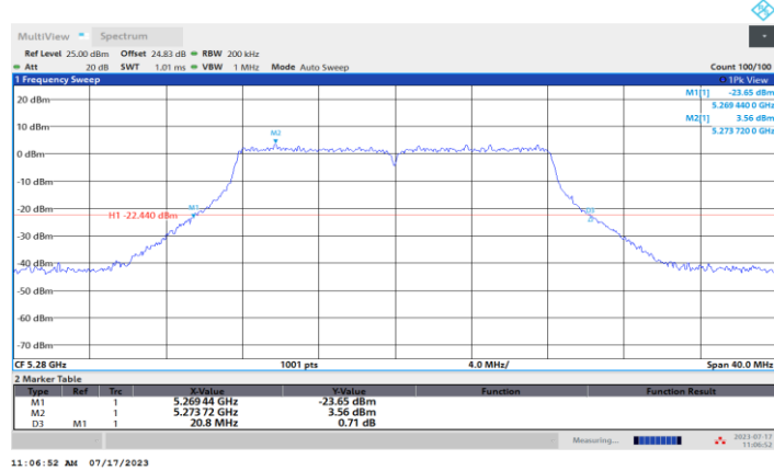
11A-CDD_Ant4_5280
