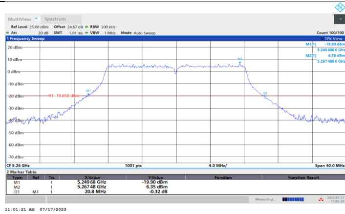
11A-CDD_Ant4_5260
