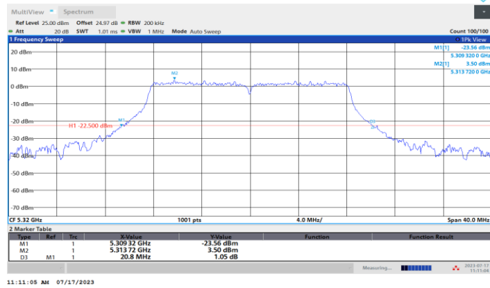
11A-CDD_Ant4_5320
