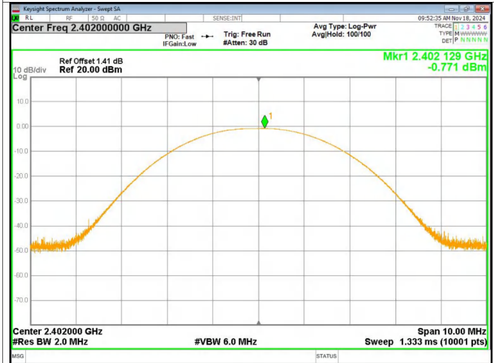
Peak Power NVNT 1-DH5 2402MHz Ant1
