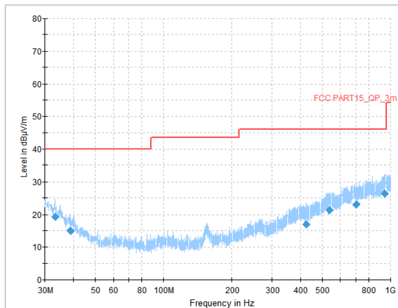
Fig.66 Radiated Spurious Emission (All Channels, 30MHz-1GHz)
