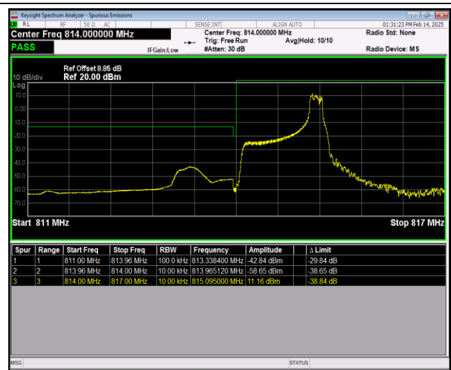
Band26-1.4MHz-64QAM-26783-1RB#0
