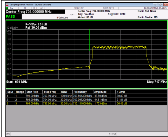
Band17-10MHz-64QAM-23800-1RB#49
