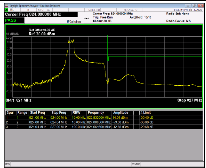
Band26-1.4MHz-16QAM-26783-6RB#0
