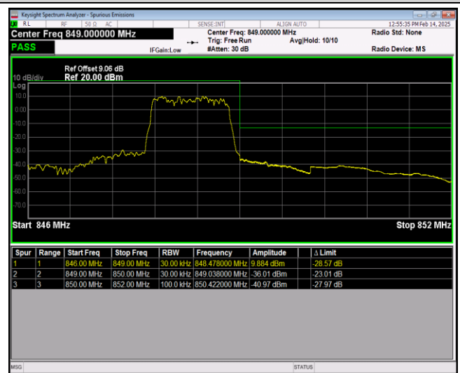
Band26-1.4MHz-16QAM-26697-1RB#5
