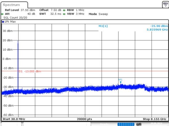
1_3MHz_Low_QPSK_15@0 -25.90dBm
