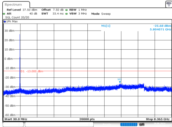
2_10MHz_Middle_QPSK_1@0 -25.68dBm
