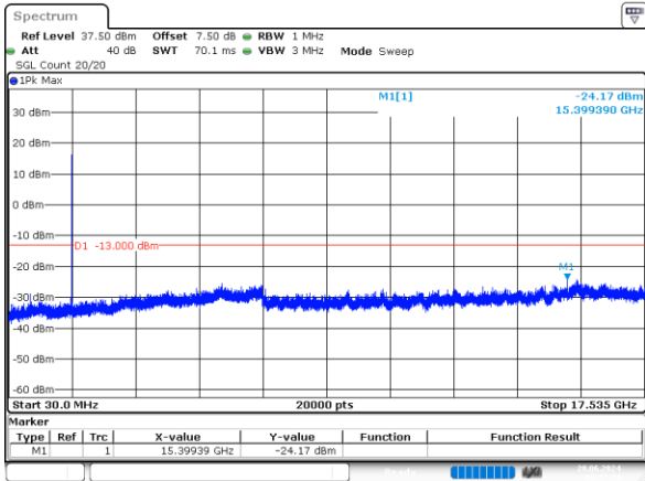
3MHz_High_QPSK_15@0 -24.17dBm
