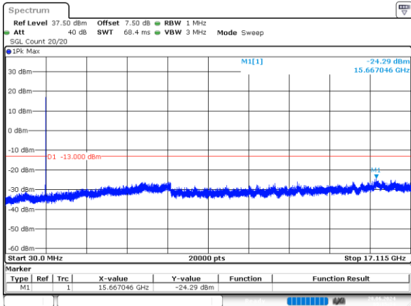
3MHz_Low_QPSK_15@0 -24.29dBm
