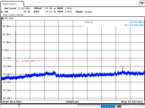
1.4MHz_Low_QPSK_6@0 -24.02dBm
