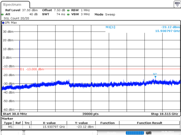
3MHz_Low_QPSK_15@0 -23.12dBm
