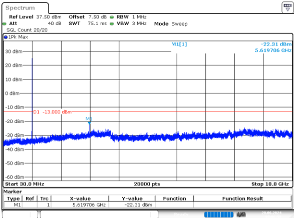
15MHz_Middle_QPSK_1@0 -22.31dBm
