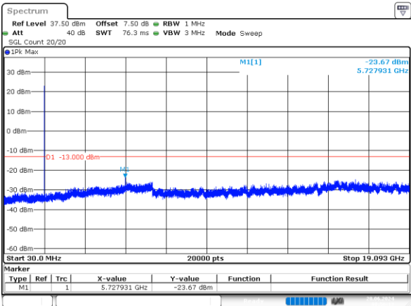
1.4MHz_High_QPSK_6@0 -23.67dBm
