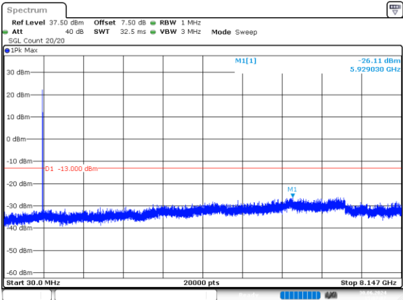
1_1.4MHz_Low_QPSK_6@0 -26.11dBm
