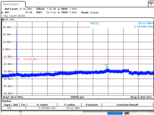
2_3MHz_Middle_QPSK_1@0 -25.41dBm
