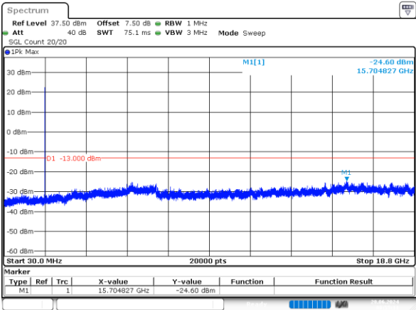
1.4MHz_Middle_QPSK_6@0 -24.60dBm
