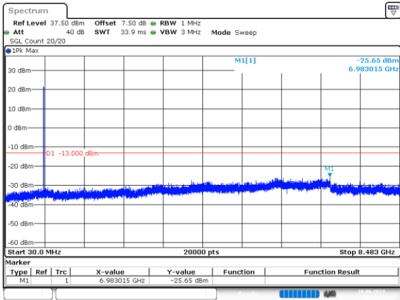
2_1.4MHz_High_QPSK_6@0 -25.65dBm
