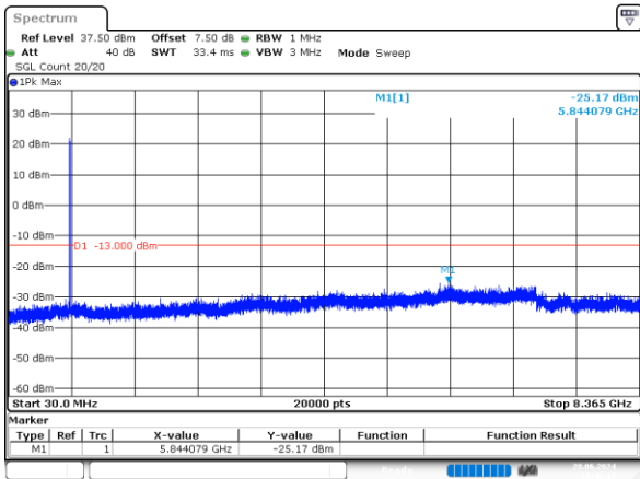
2_1.4MHz_Middle_QPSK_6@0 -25.17dBm
