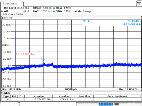
3MHz_High_QPSK_15@0 -24.45dBm
