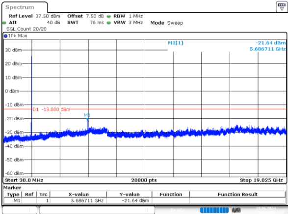
15MHz_High_QPSK_1@0 -21.64dBm
