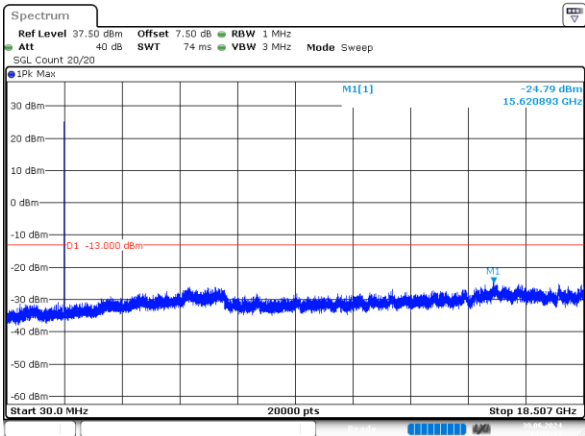
1.4MHz_Low_QPSK_1@0 -24.79dBm
