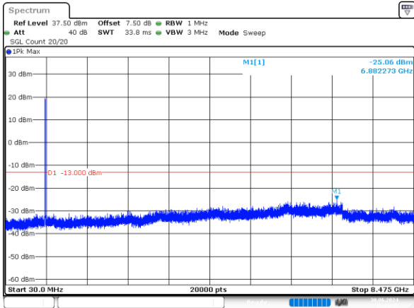
2_3MHz_High_QPSK_15@0 -25.06dBm
