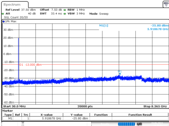
2_3MHz_Middle_QPSK_15@0 -25.80dBm
