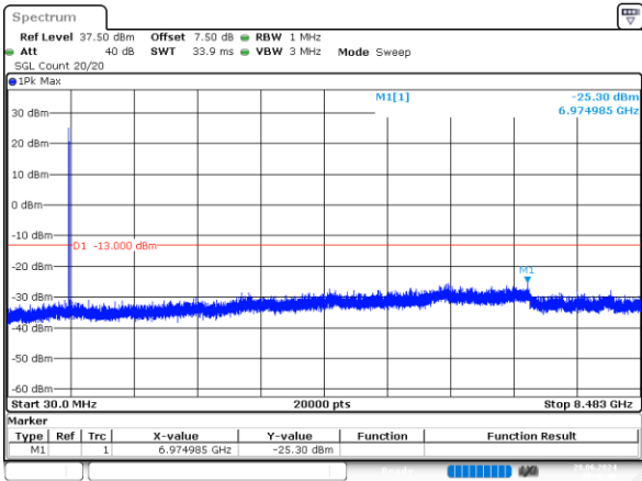
2_1.4MHz_High_QPSK_1@0 -25.30dBm
