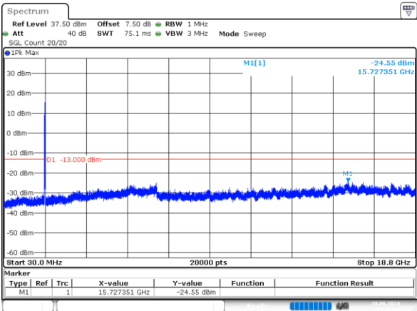
20MHz_Middle_QPSK_100@0 -24.55dBm
