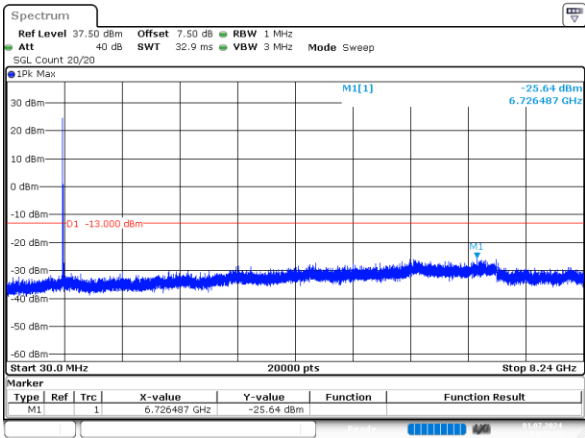
3_10MHz_Middle_QPSK_1@0 -25.64dBm
