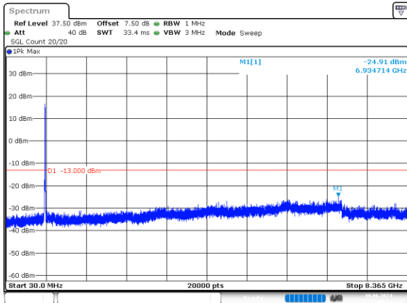
2_15MHz_Middle_QPSK_75@0 -24.91dBm
