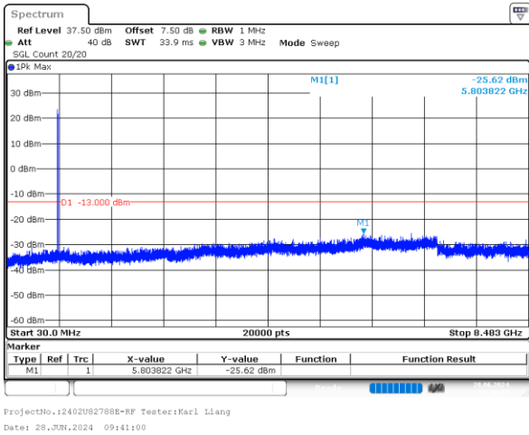
1.4MHz_High_QPSK_6@0 -25.62dBm
