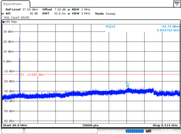
1_5MHz_High_QPSK_1@0 -25.72dBm
