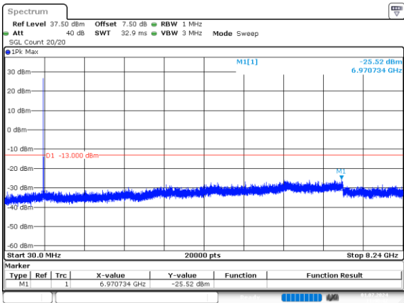
3_5MHz_Middle_QPSK_1@0 -25.52dBm
