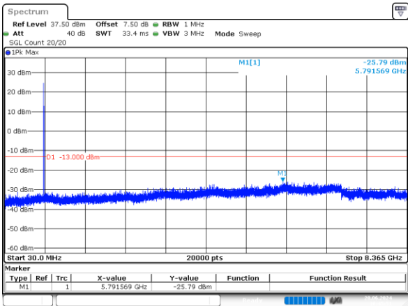
2_1.4MHz_Middle_QPSK_1@0 -25.79dBm
