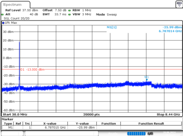
10MHz_High_QPSK_50@0 -25.99dBm
