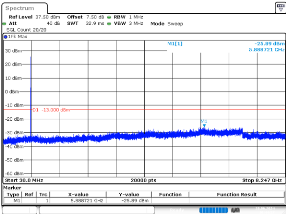
2_1.4MHz_Low_QPSK_1@0 -25.89dBm
