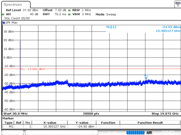
5MHz_High_QPSK_25@0 -24.92dBm
