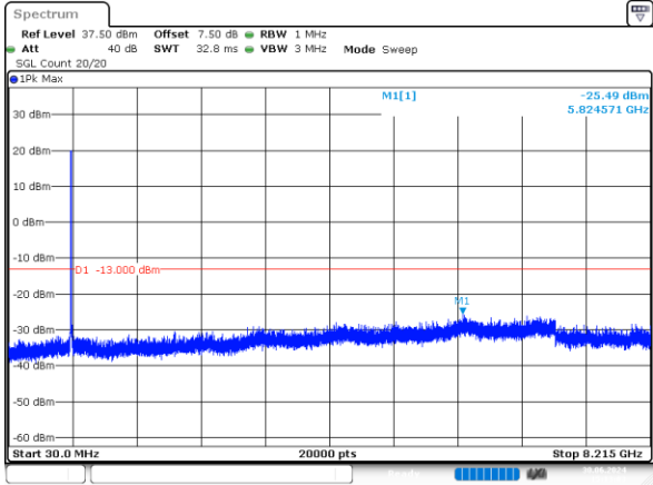
1_5MHz_High_QPSK_25@0 -25.49dBm
