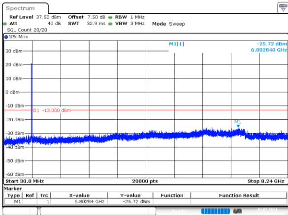
3_3MHz_Middle_QPSK_15@0 -25.72dBm
