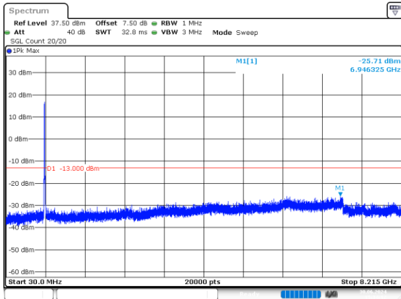
1_15MHz_Low_QPSK_75@0 -25.71dBm
