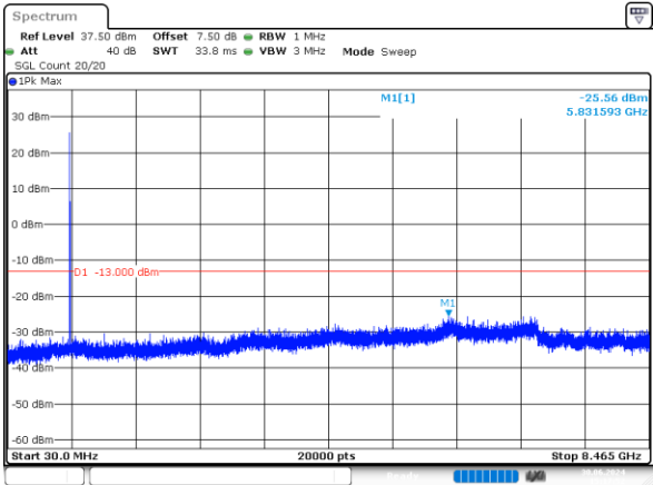
2_5MHz_High_QPSK_1@0 -25.56dBm
