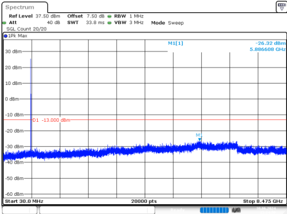
2_3MHz_High_QPSK_1@0 -26.32dBm
