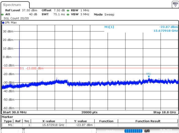
3MHz_Middle_QPSK_15@0 -23.87dBm
