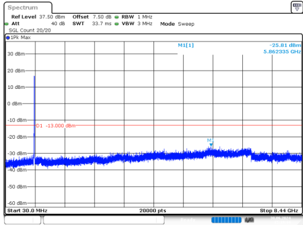
2_10MHz_High_QPSK_50@0 -25.81dBm
