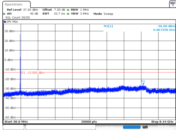
2_10MHz_High_QPSK_1@0 -26.00dBm
