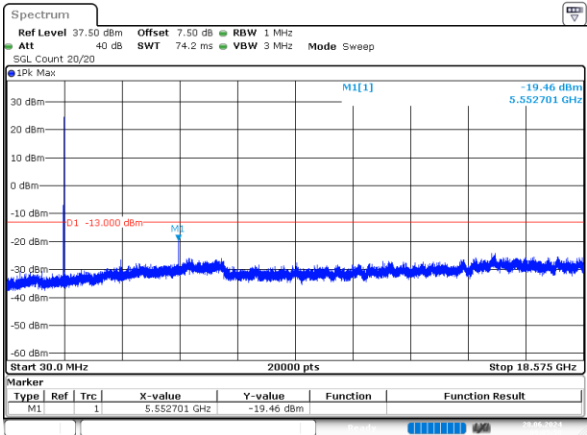
15MHz_Low_QPSK_1@0 -19.46dBm
