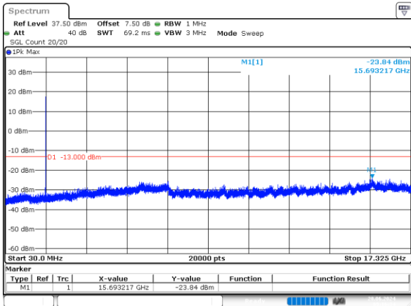
3MHz_Middle_QPSK_15@0 -23.84dBm
