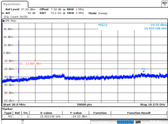
15MHz_Low_QPSK_75@0 -24.22dBm
