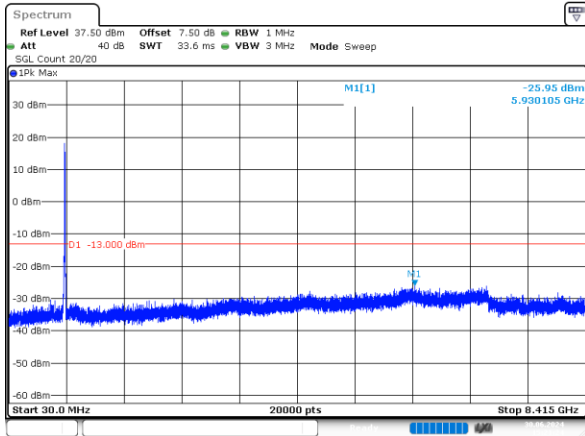
2_15MHz_High_QPSK_75@0 -25.95dBm
