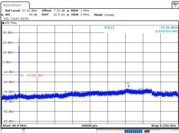
1_1.4MHz_High_QPSK_6@0 -25.36dBm
