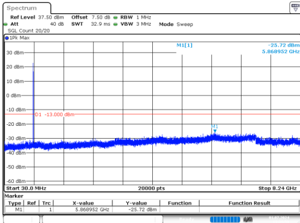
3_1.4MHz_Middle_QPSK_6@0 -25.72dBm
