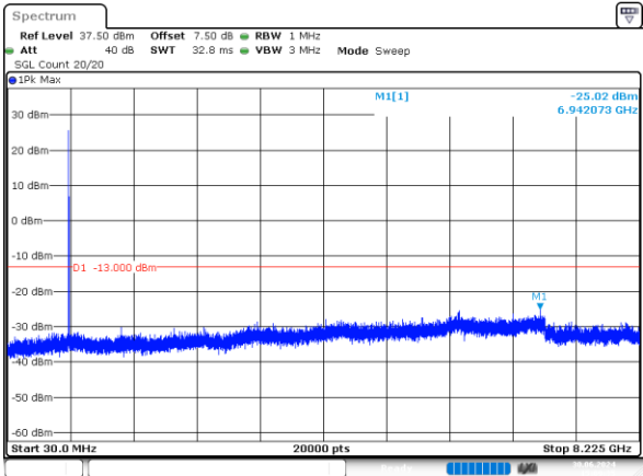
1_3MHz_High_QPSK_1@0 -25.02dBm
