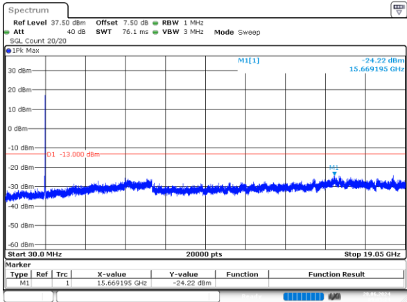
10MHz_High_QPSK_50@0 -24.22dBm
