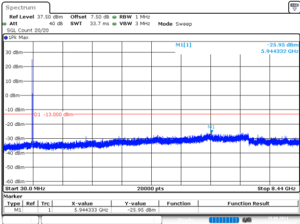
10MHz_High_QPSK_1@0 -25.95dBm
