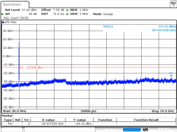
20MHz_High_QPSK_100@0 -24.15dBm
