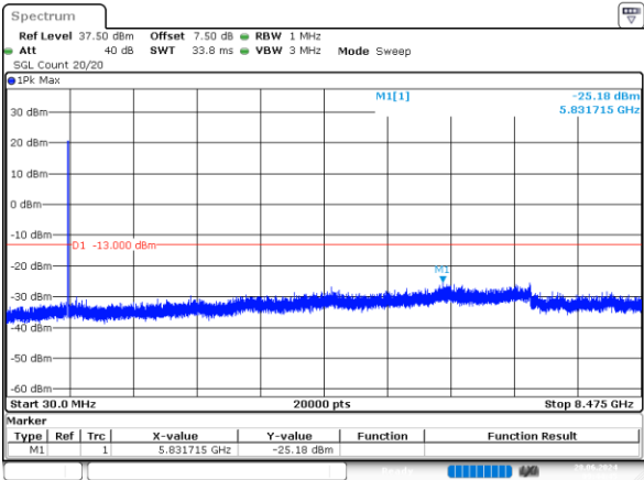
3MHz_High_QPSK_15@0 -25.18dBm
