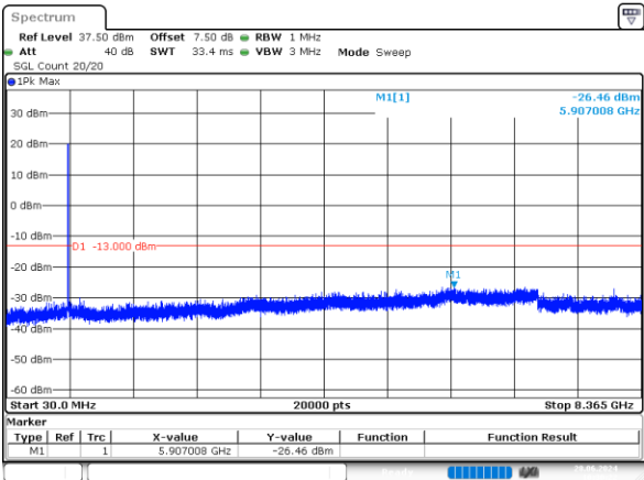
3MHz_Middle_QPSK_15@0 -26.46dBm
