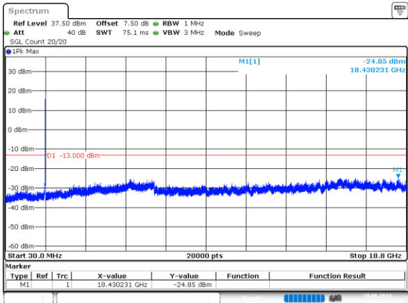
15MHz_Middle_QPSK_75@0 -24.85dBm
