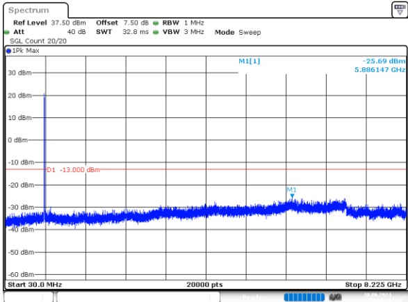
1_3MHz_High_QPSK_15@0 -25.69dBm
