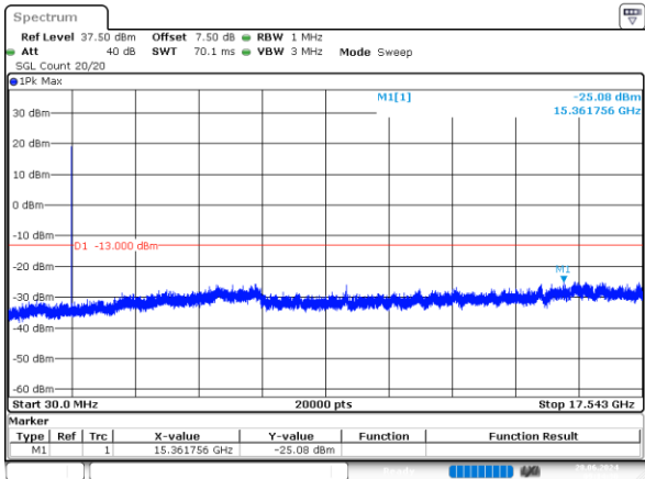
1.4MHz_High_QPSK_6@0 -25.08dBm
