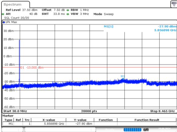
5MHz_High_QPSK_25@0 -27.90dBm
