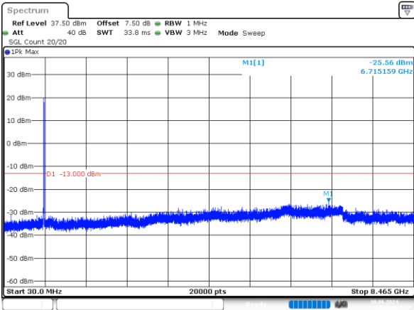
2_5MHz_High_QPSK_25@0 -25.56dBm
