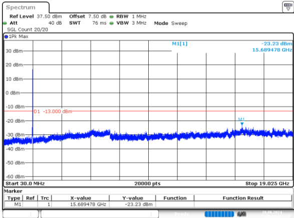
15MHz_High_QPSK_75@0 -23.23dBm
