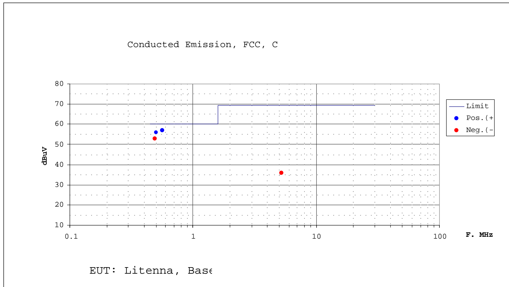
Fig. 1 Conducted Emission vrs. FCC Class A Standard Limit, \pm 48\text{VDC} Power Supply of the Base Unit, Q.P. Detector.
