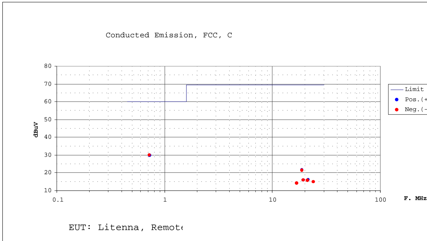
Fig. 2 Conducted Emission vrs. FCC Class A Standard Limit, \pm 48 VDC Power Supply of the Remote Unit, Q.P. Detector.
