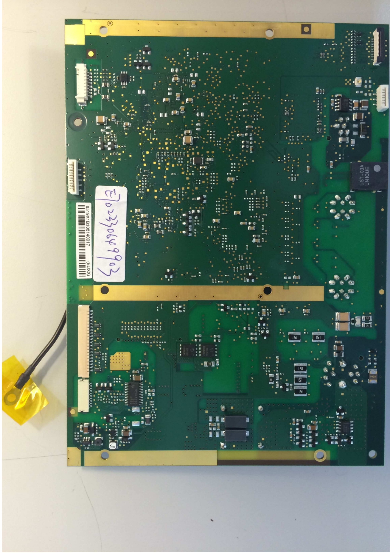
Figure 2 - CPU_PCBA_BOTTOM
