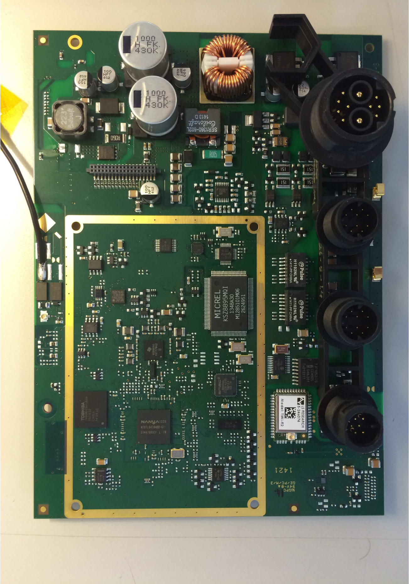
Figure 3 - CPU_PCBA_TOP
