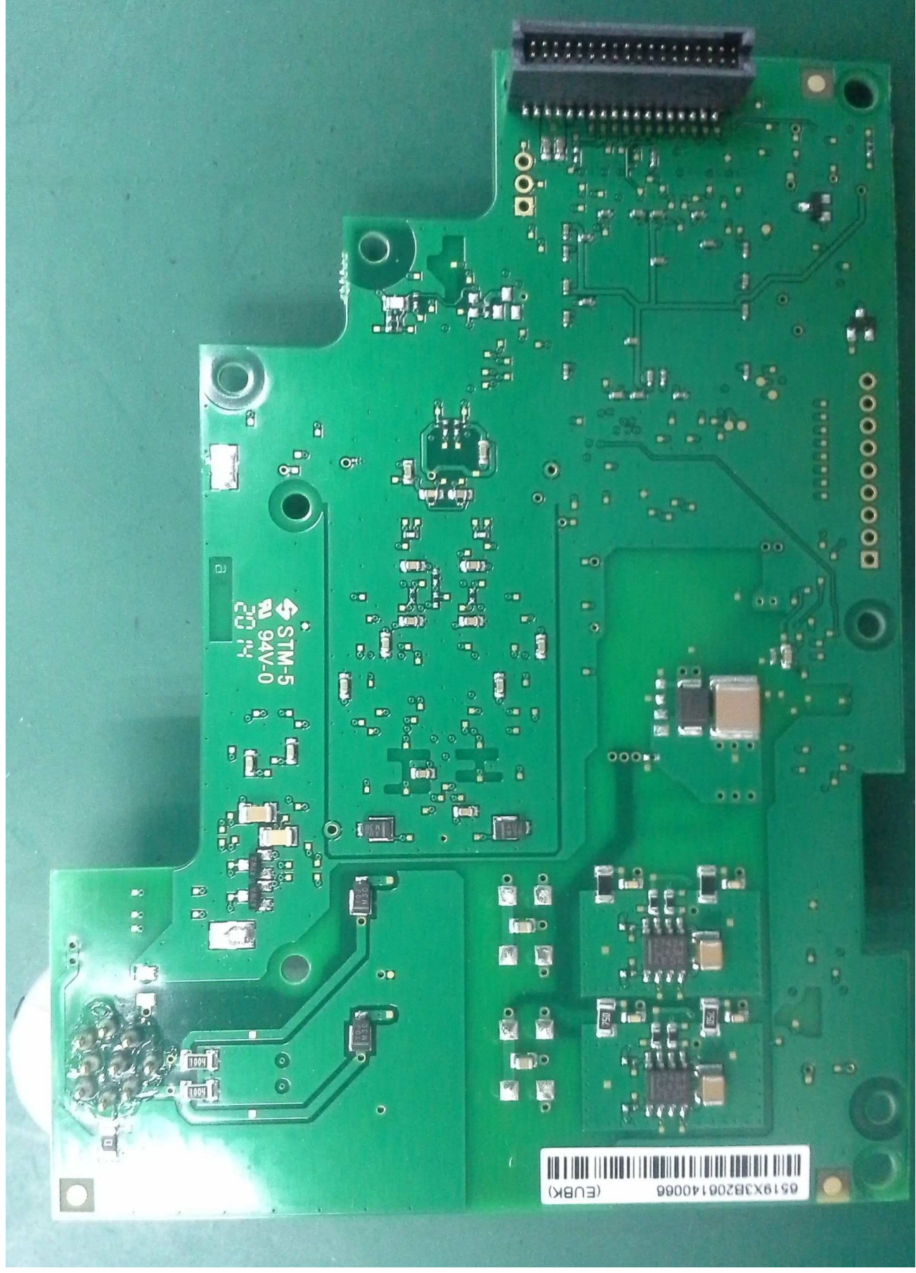
Figure 4 - DOWNVISION_PCBA_BOTTOM
