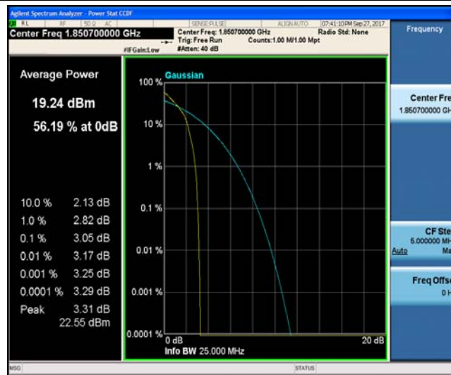
Band2_1.4MHz_16QAM_18607_1RB#0_3.78_13_PASS
