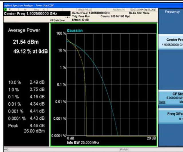
Band2_15MHz_16QAM_19125_1RB#0_4.73_13_PASS
