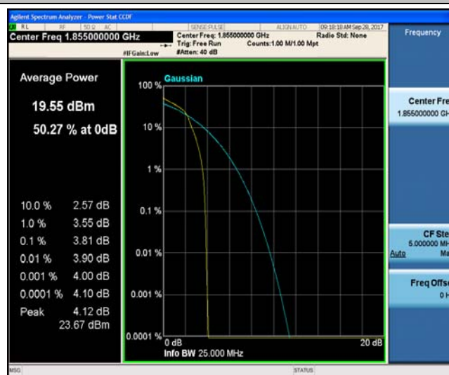
Band2_10MHz_QPSK_18650_50RB#0_4.30_13_PASS
