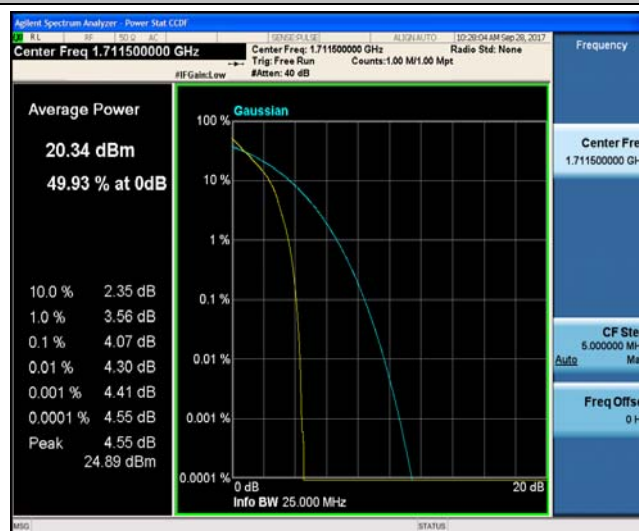
Band4_3MHz_16QAM_19965_15RB#0_5.59_13_PASS
