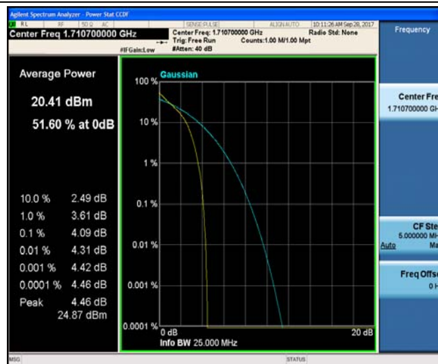
Band4_1.4MHz_16QAM_19957_6RB#0_5.71_13_PASS
