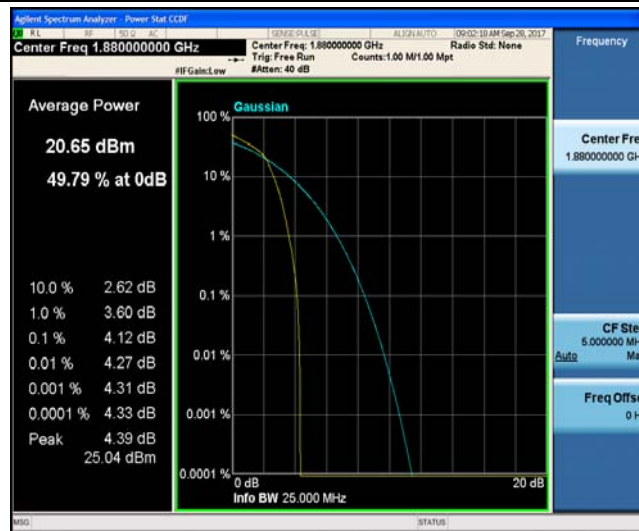
Band2_5MHz_QPSK_18900_25RB#0_4.16_13_PASS
