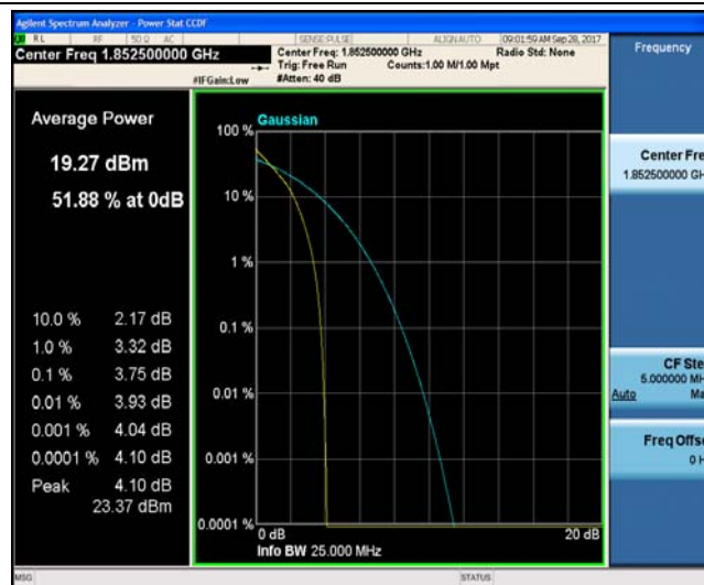
Band2_5MHz_16QAM_18625_25RB#0_5.48_13_PASS
