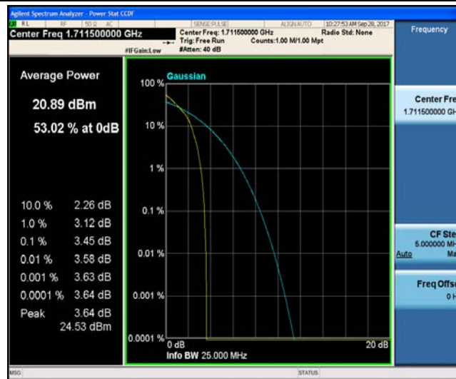
Band4_3MHz_16QAM_19965_1RB#0_4.18_13_PASS
