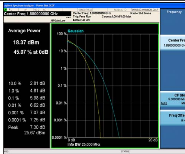
Band2_20MHz_QPSK_18900_1RB#0_3.90_13_PASS
