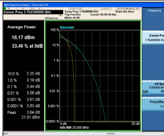
Band4_1.4MHz_16QAM_20393_1RB#0_4.04_13_PASS
