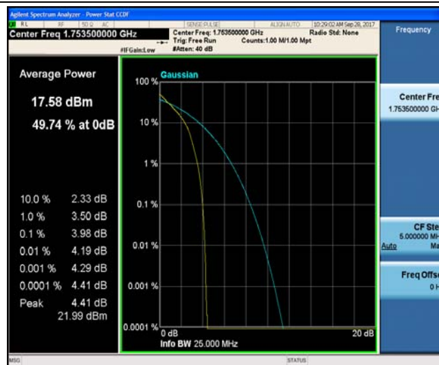
Band4_3MHz_16QAM_20385_15RB#0_5.72_13_PASS
