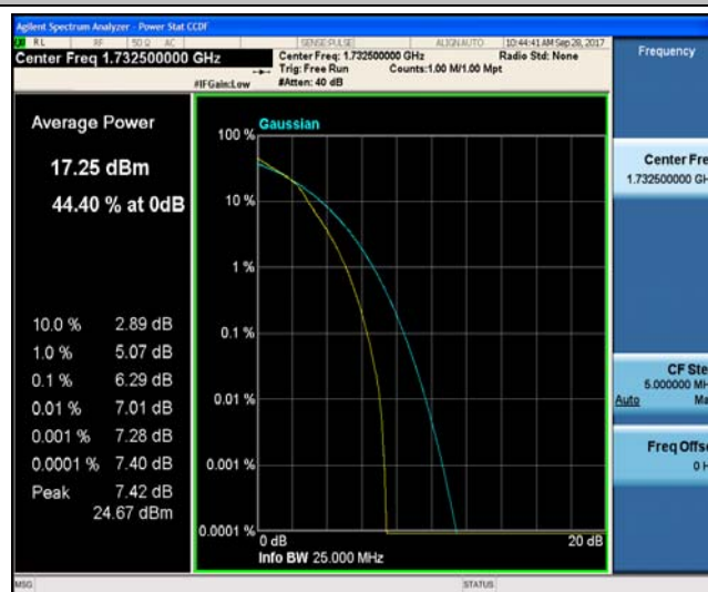
Band4_5MHz_QPSK_20375_1RB#0_2.92_13_PASS
