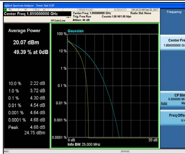
Band2_10MHz_16QAM_18650_50RB#0_5.90_13_PASS
