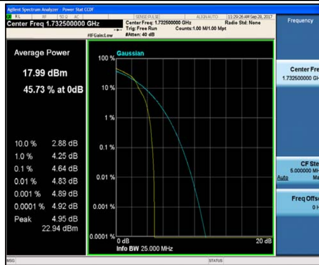
Band4_10MHz_QPSK_20175_50RB#0_4.60_13_PASS
