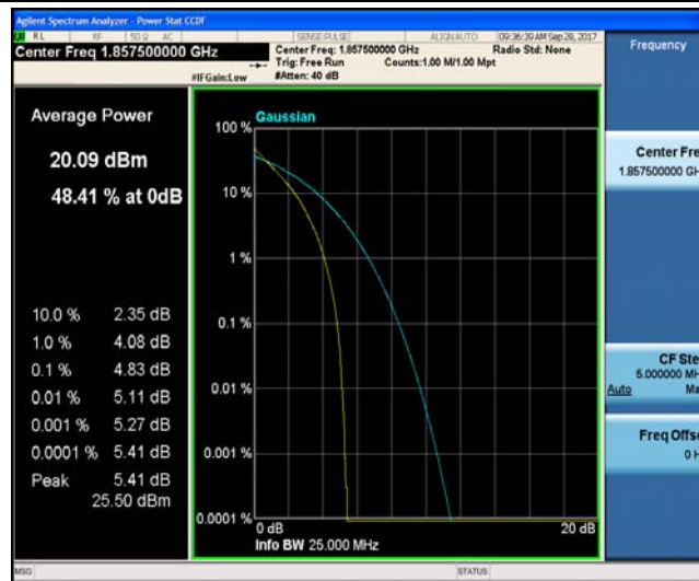
Band2_15MHz_16QAM_18675_75RB#0_6.14_13_PASS
