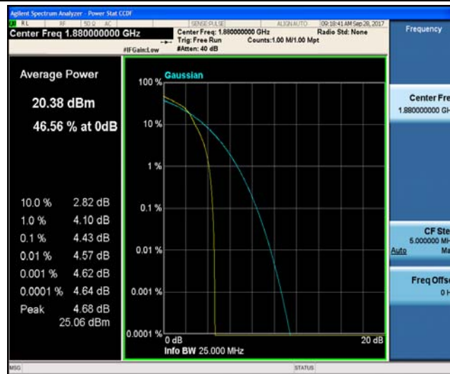
Band2_10MHz_QPSK_18900_50RB#0_4.10_13_PASS
