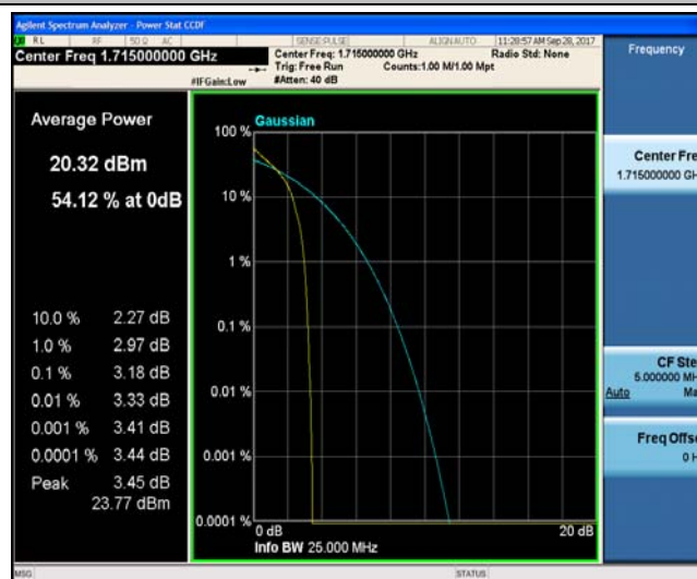
Band4_10MHz_16QAM_20000_1RB#0_4.16_13_PASS
