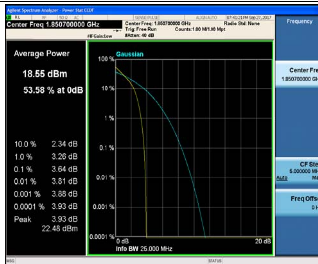
Band2_1.4MHz_16QAM_18607_6RB#0_5.35_13_PASS
