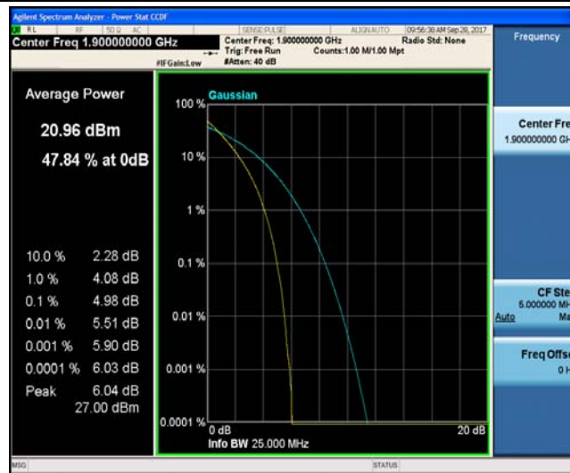
Band2_20MHz_16QAM_19100_100RB#0_6.18_13_PASS
