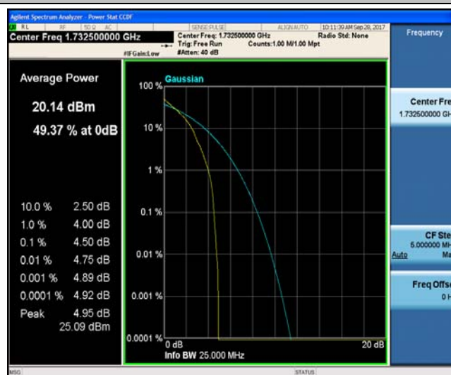
Band4_1.4MHz_16QAM_20175_1RB#0_5.69_13_PASS
