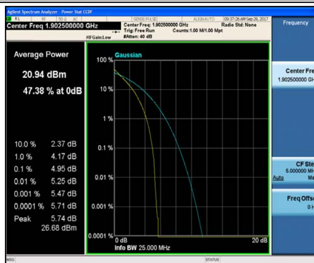
Band2_15MHz_16QAM_19125_75RB#0_6.23_13_PASS
