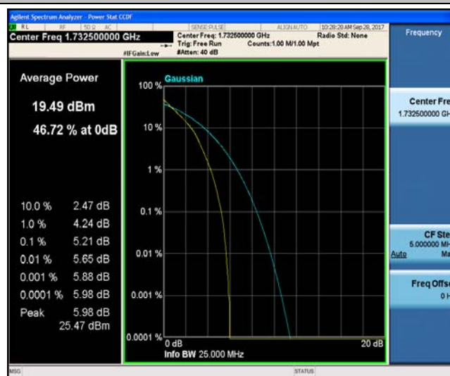
Band4_3MHz_16QAM_20175_15RB#0_6.43_13_PASS
