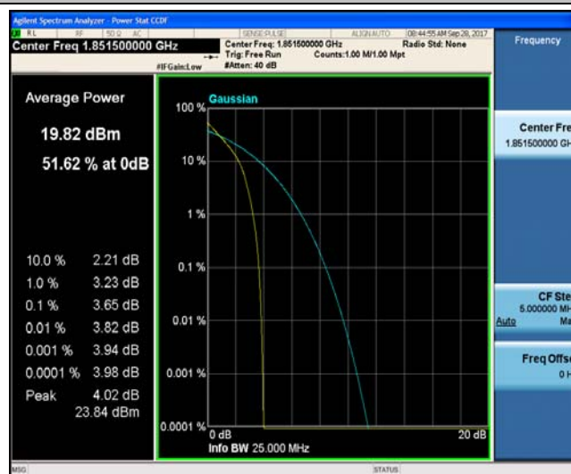
Band2_3MHz_16QAM_18615_15RB#0_5.30_13_PASS
