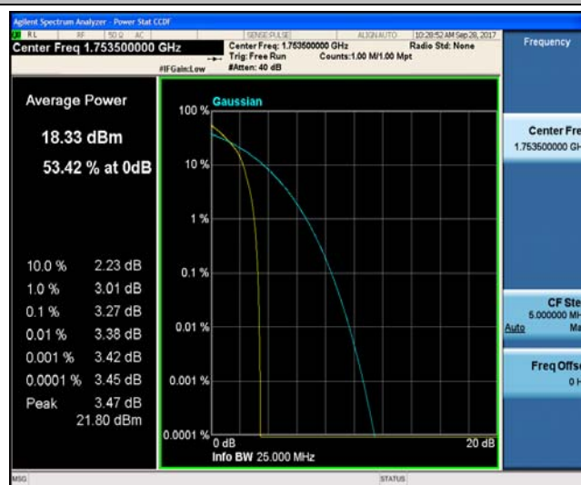
Band4_3MHz_16QAM_20385_1RB#0_3.80_13_PASS
