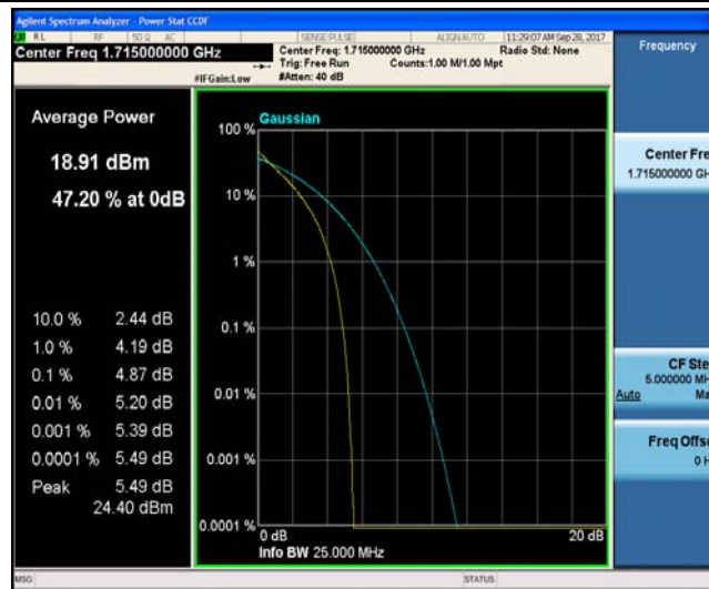
Band4_10MHz_16QAM_20000_50RB#0_5.70_13_PASS
