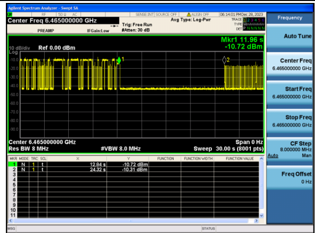
802.11be-HET80 / CH103 (High Edge)
