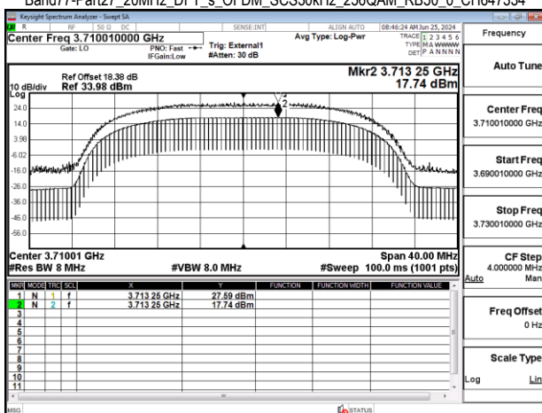
Band77-Part27_20MHz_DFT_s_OFDM_SCS30kHz_256QAM_RB50_0_CH647334
