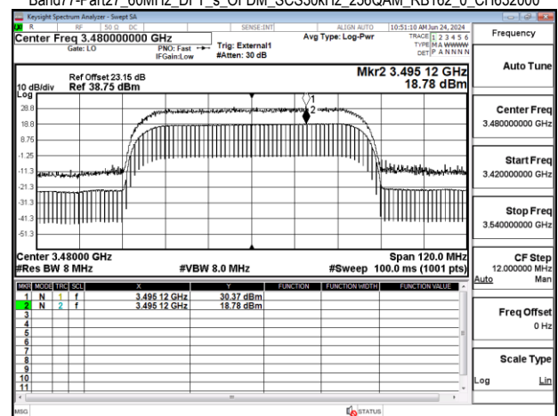
Band77-Part27 60MHz DFT s OFDM_SCS30kHz 256QAM_RB162_0_CH632000
