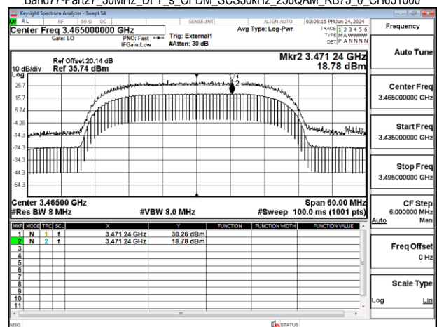
Band77-Part27_30MHz_DFT_s_OFDM_SCS30kHz_256QAM_RB75_0_CH631000
