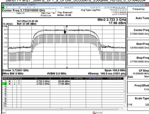
Band77-Part27 50MHz DFT s OFDM_SCS30kHz 256QAM_RB128_0_CH648334
