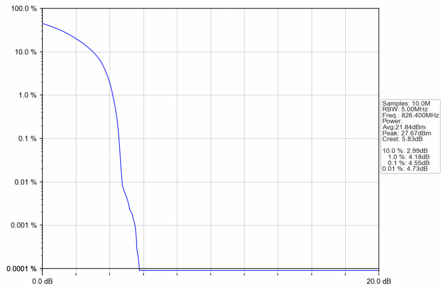
Band5_HSUPA_LCH_826.4MHz_Subtest 1_NTNV
