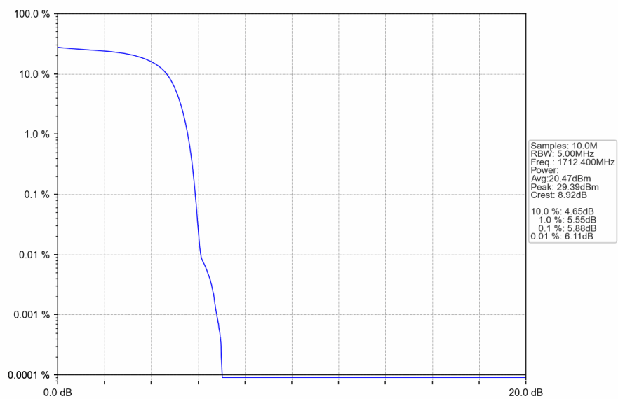
Band4_HSDPA_LCH_1712.4MHz_Subtest 1_NTNV
