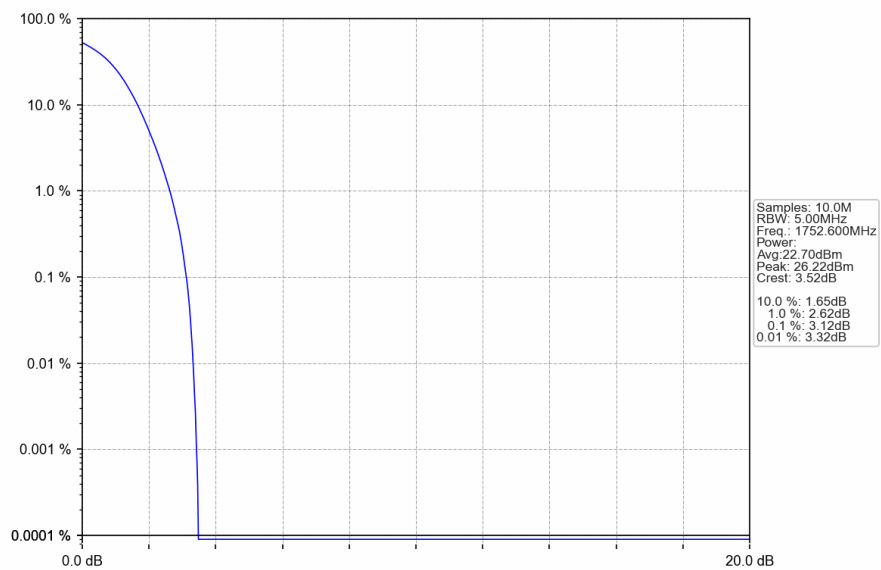
Band4_RMC_HCH_1752.6MHz_12.2kbps RMC_NTNV
