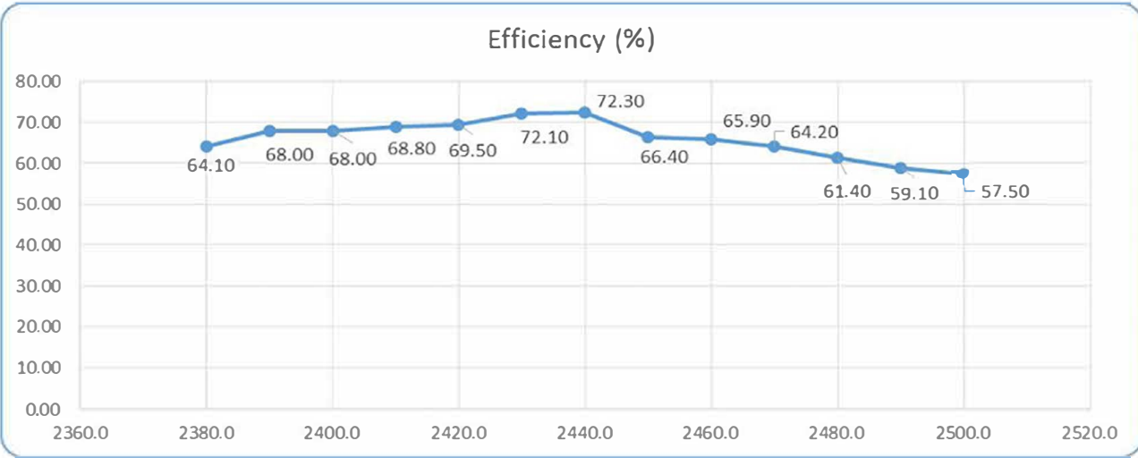
◎ 效率 efficiency
