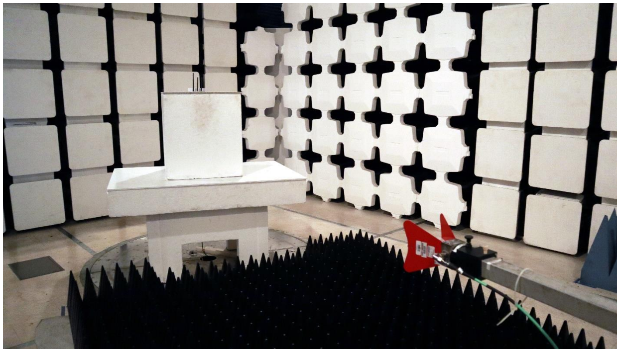
Co Location Spurious Emissions 1-18GHz
