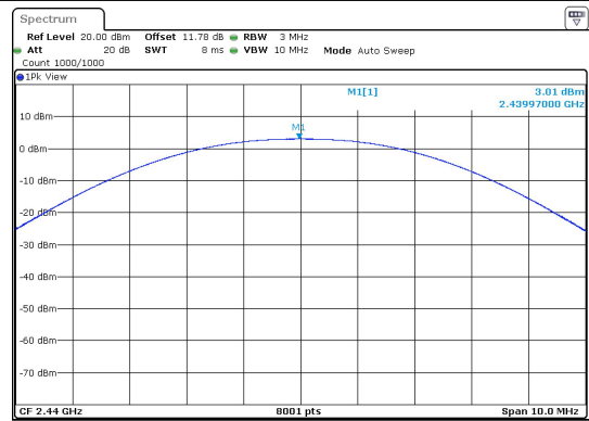
BLE_1M-Ant1-2440-PASS
