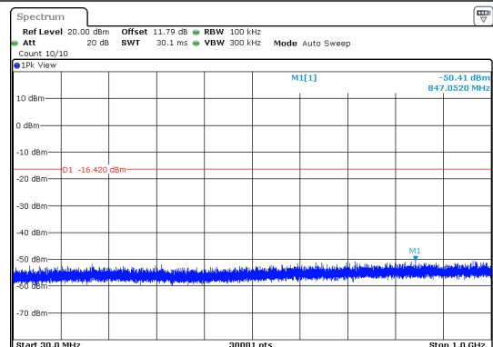
BLE_1M-Ant1-2480-30~1000-PASS
