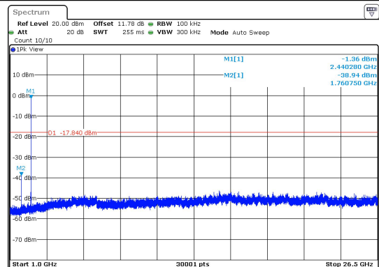
BLE_1M-Ant1-2440-1000~26500-PASS
