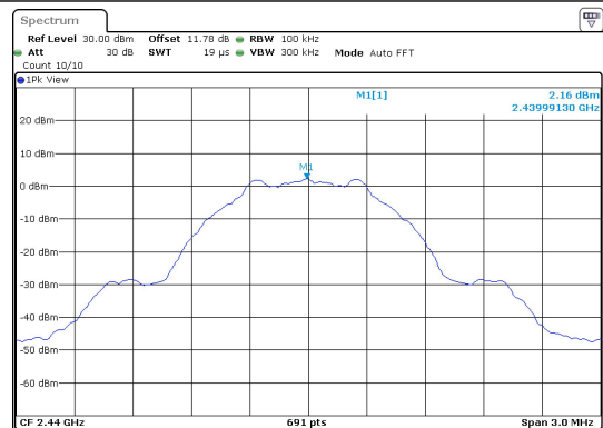
BLE_1M-Ant1-2440-0~Reference-PASS
