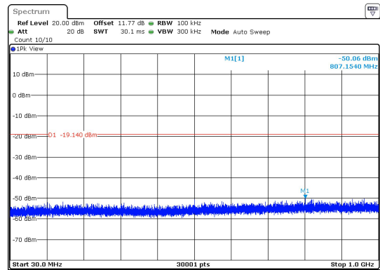
BLE_1M-Ant1-2402-30~1000-PASS
