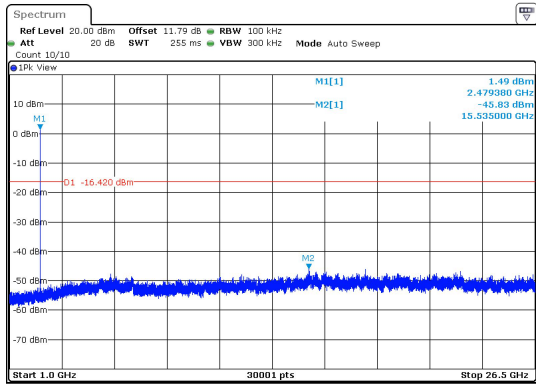
BLE_1M-Ant1-2480-1000~26500-PASS
