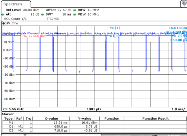
NTNV-11AC40-CDD-Ant1-5550
