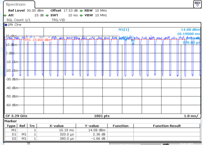
NTNV-11AC80-CDD-Ant2-5290
