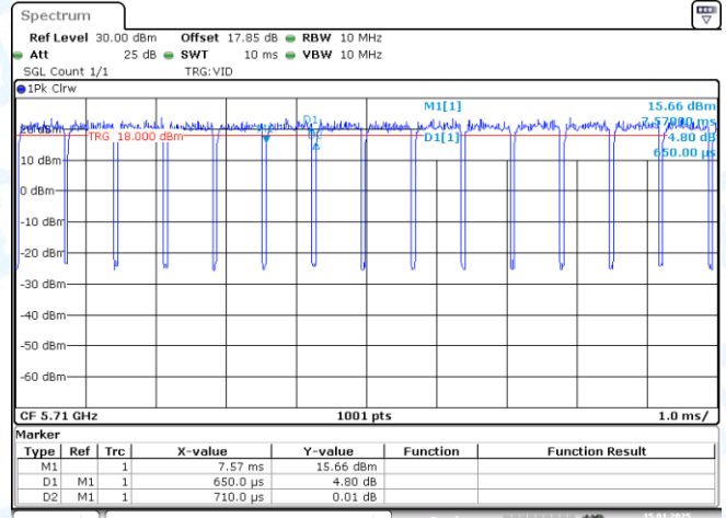
NTNV-11N40-CDD-Ant2-5710
