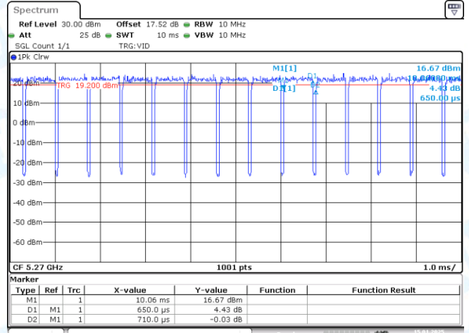
NTNV-11AC40-CDD-Ant2-5270
