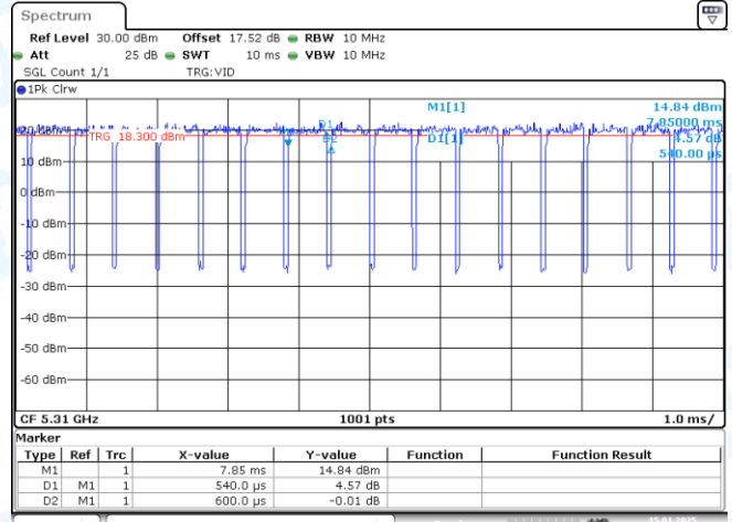
NTNV-11AX40-CDD-Ant2-5310
