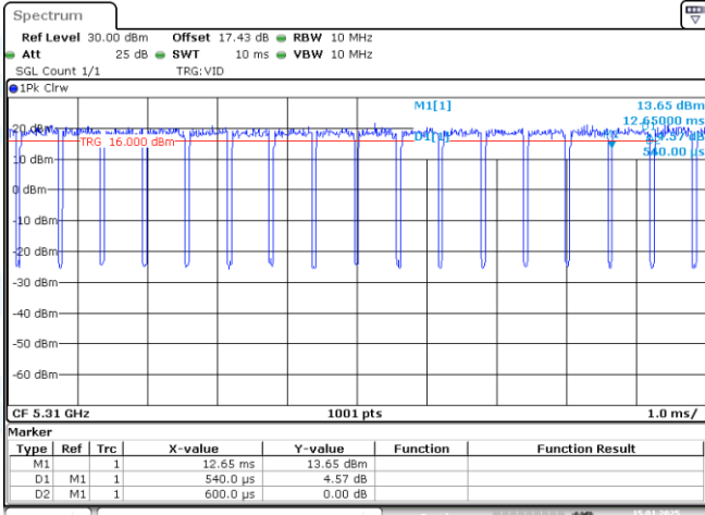
NTNV-11AX40-CDD-Ant1-5310
