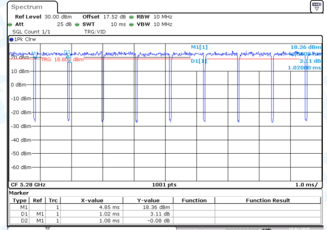
NTNV-11AX20-CDD-Ant2-5280
