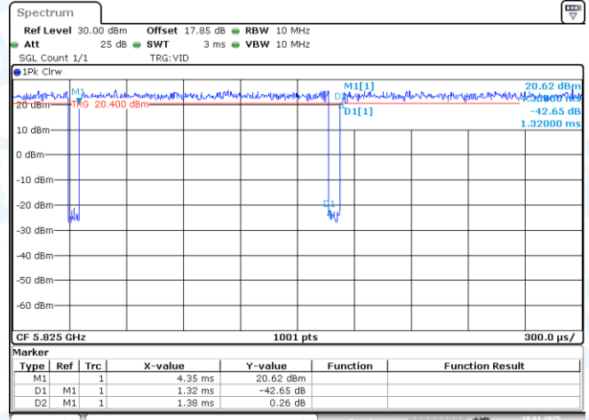
NTNV-11AC20-CDD-Ant2-5825
