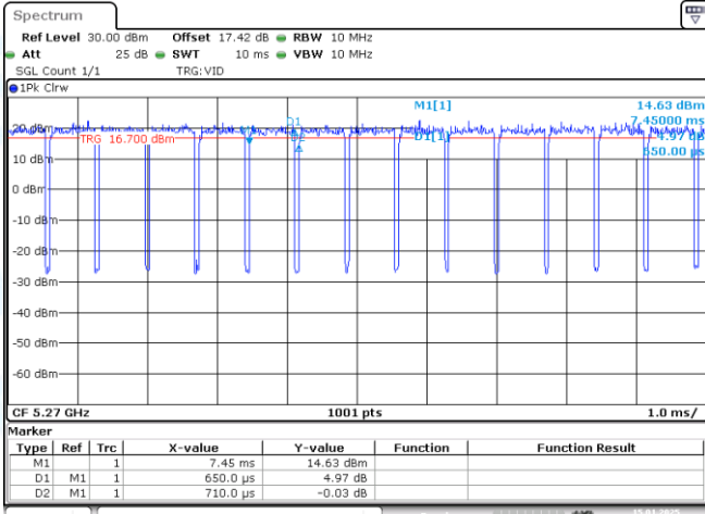
NTNV-11AC40-CDD-Ant1-5270
