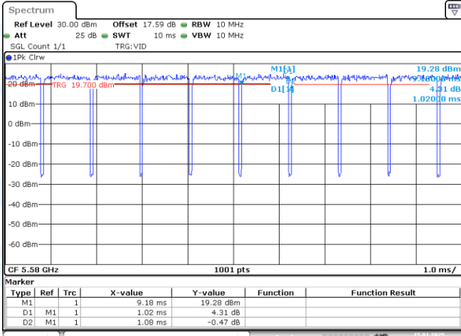
NTNV-11AX20-CDD-Ant1-5580
