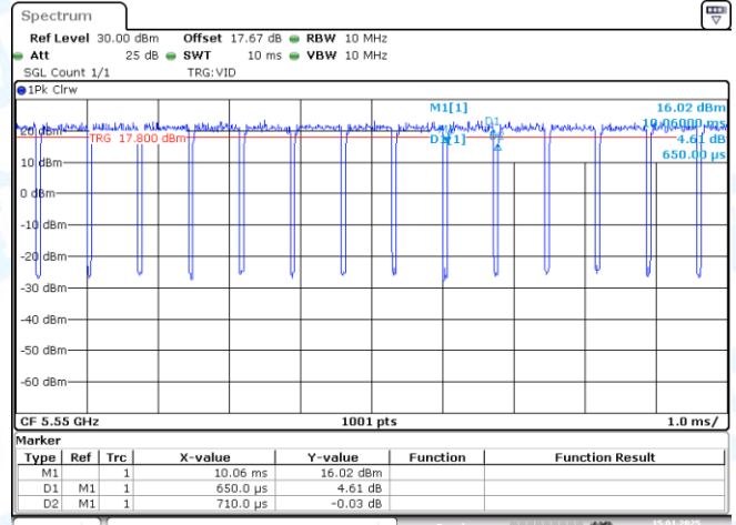
NTNV-11AC40-CDD-Ant2-5550
