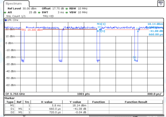
NTNV-11AC40-CDD-Ant2-5755
