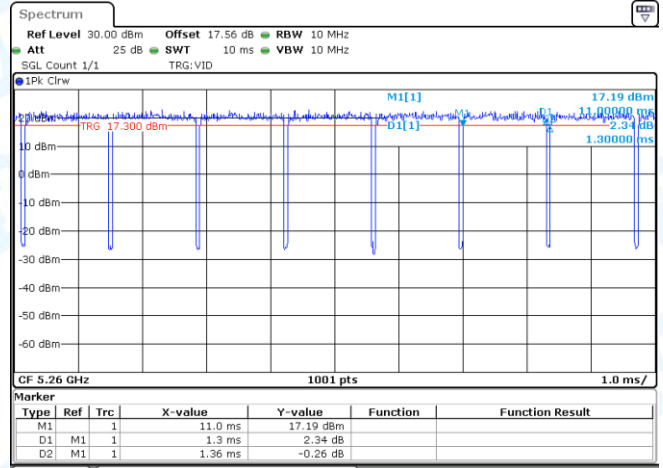
NTNV-11AC20-CDD-Ant2-5260
