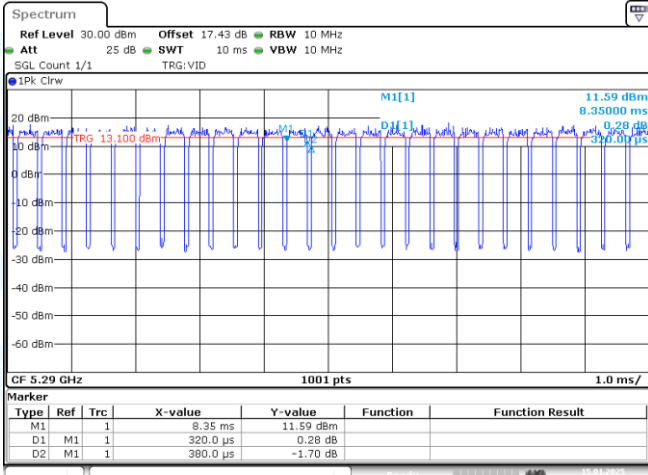
NTNV-11AC80-CDD-Ant1-5290
