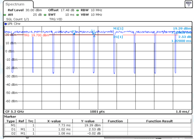
NTNV-11AX20-CDD-Ant2-5200
