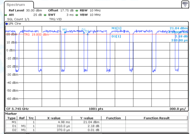
NTNV-11AX20-CDD-Ant2-5745
