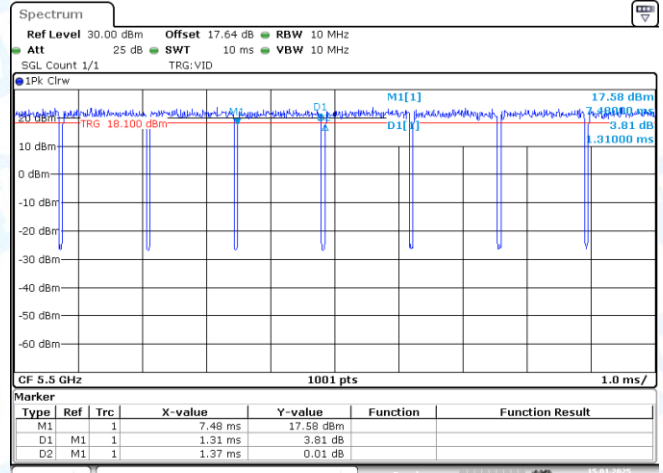
NTVN-11AC20-CDD-Ant2-5500
