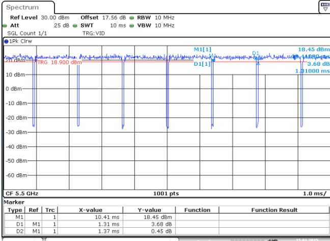
NTVN-11AC20-CDD-Ant1-5500
