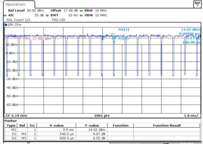
NTNV-11AX40-CDD-Ant2-5190
