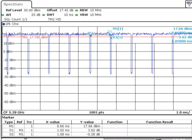
NTNV-11AX20-CDD-Ant1-5280
