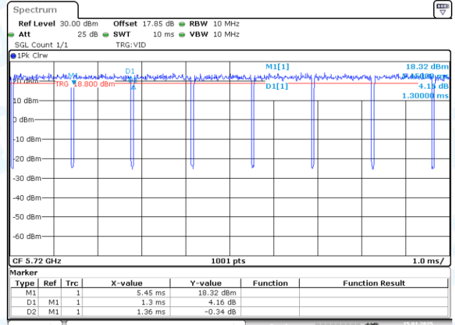
NTNV-11AC20-CDD-Ant2-5720
