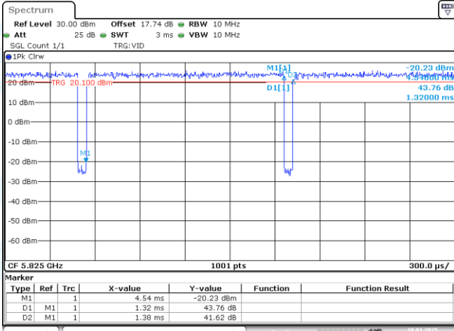
NTNV-11AC20-CDD-Ant1-5825
