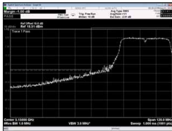
Channel 38 (5190MHz)
