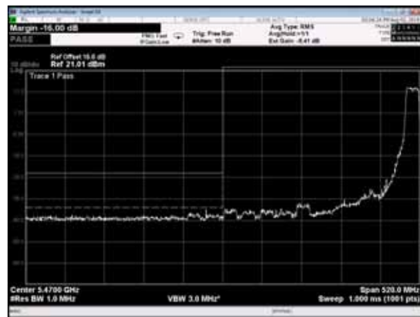
Channel 144 (5720MHz)
