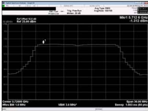
Channel 144 (5720MHz)
