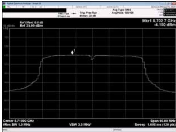
Channel 142 (5710MHz)
