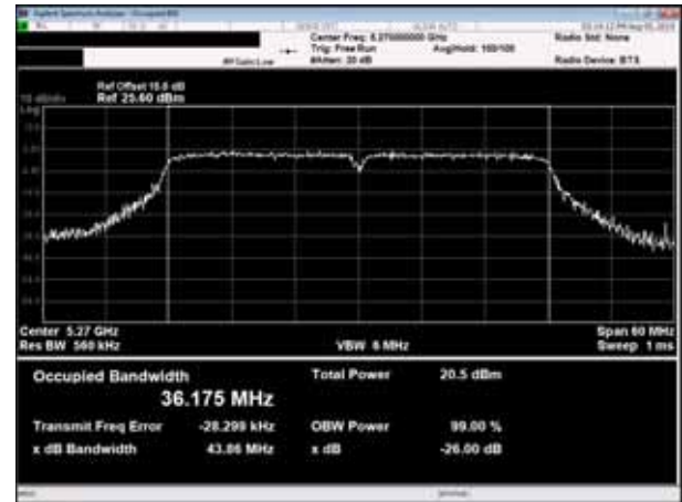
Channel 54 (5270MHz)
