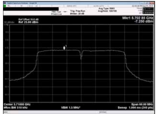
Channel 142 (5710MHz)
