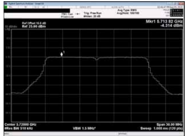
Channel 144 (5720MHz)
