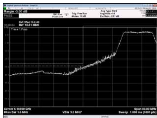
Channel 36 (5180MHz)
