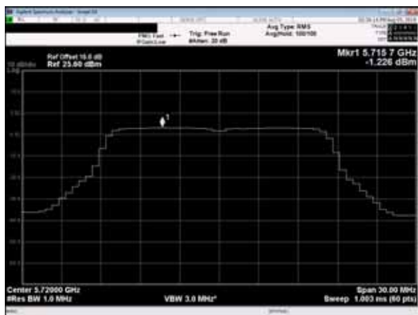
Channel 144 (5720MHz)
