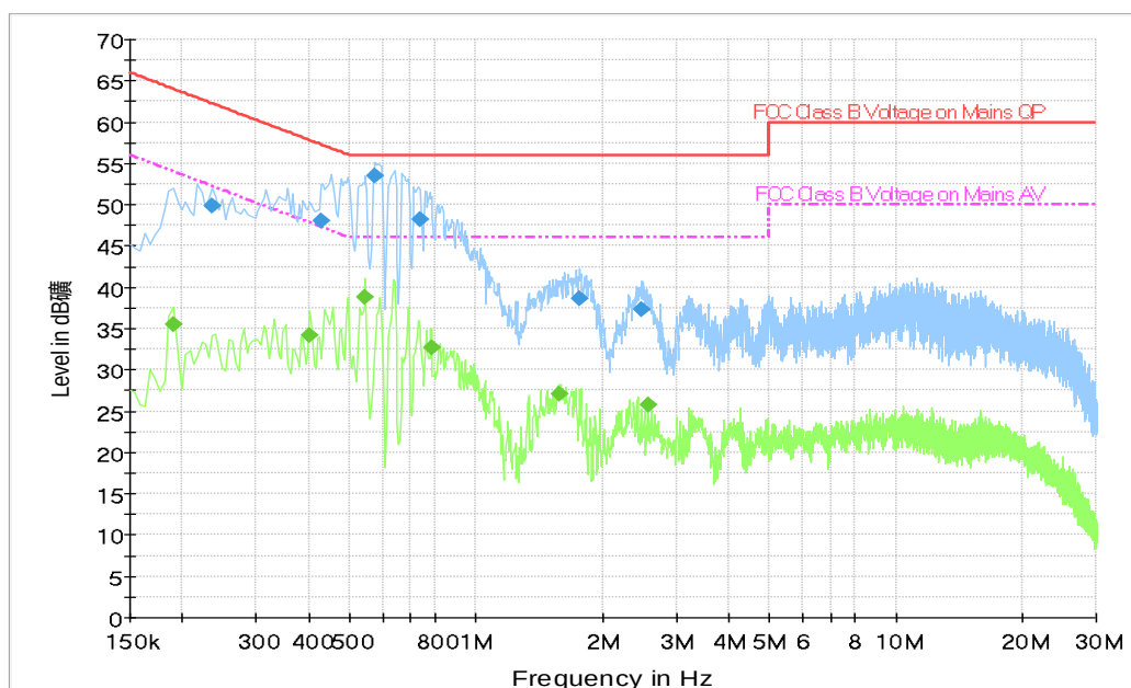
Fig. 22 AC Power line Conducted Emission-802.11a
