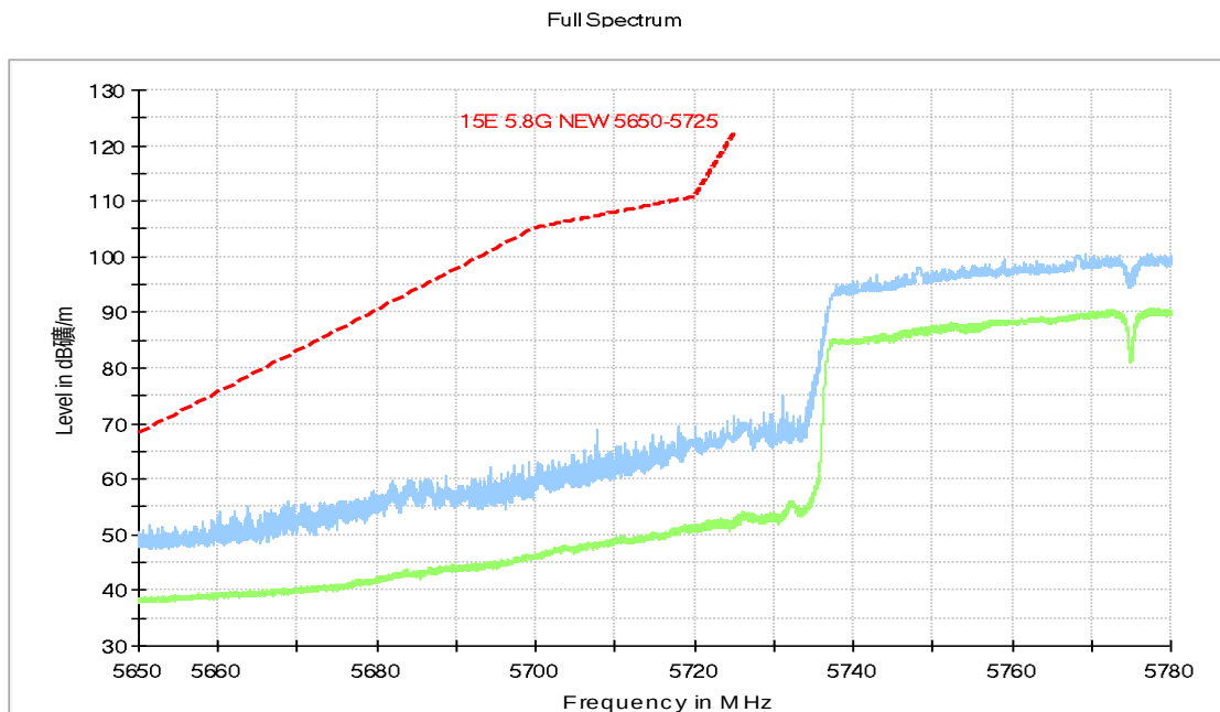
Fig. 20 Band Edges (802.11ac-HT80 Ch155, 5775MHz)
