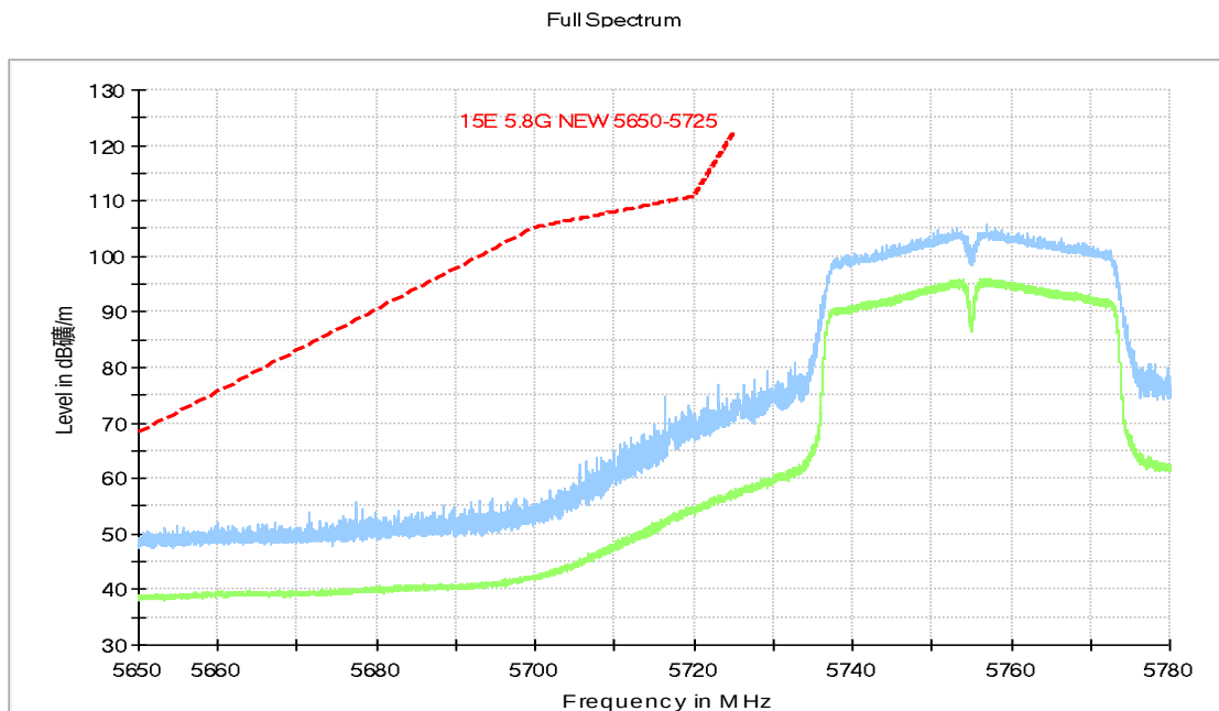
Fig. 18 Band Edges (802.11ac-HT40 Ch151, 5755MHz)
