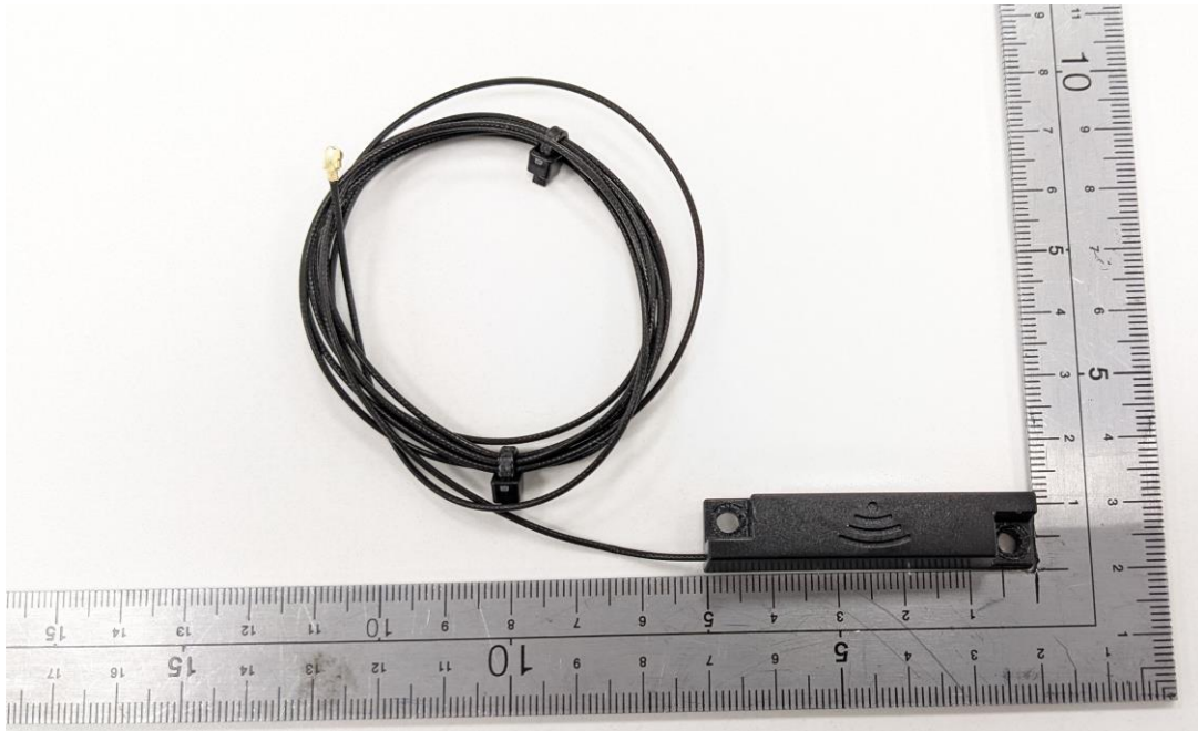
Antenna 0 & 1
