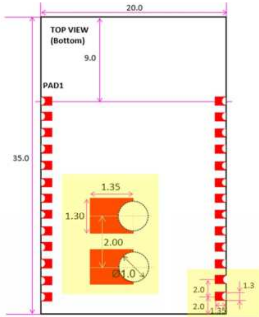
Figure 4-1 Module Dimension
