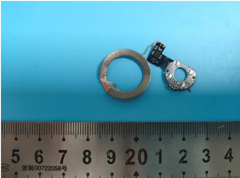
WPT Coil (RX only)
