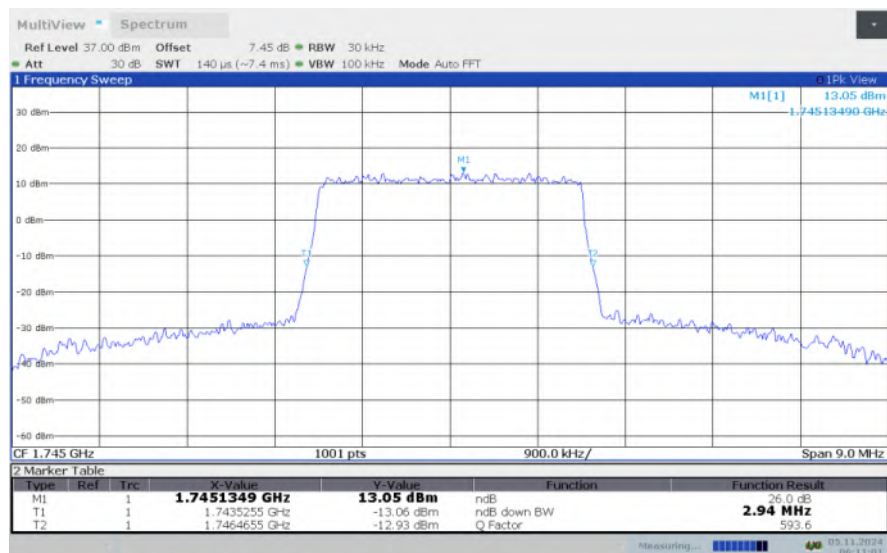
LTE band 66 , 3MHz Bandwidth, MID, QPSK (-26dBc BW)
