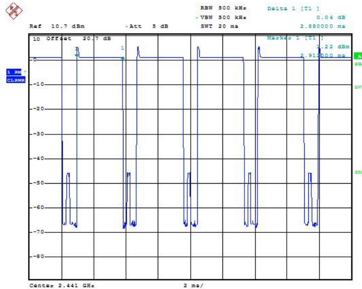
Fig.75 Number of Transmissions Measurement: Ch39, Packet 3-DH3
