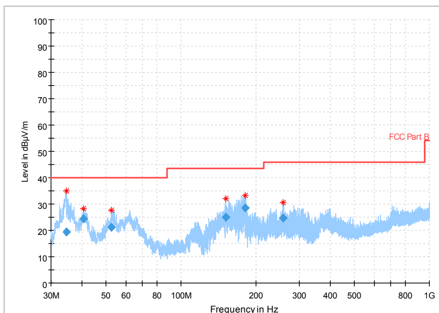
Fig.55 Radiated emission: \pi/4 DQPSK, Ch78, 30MHz~1GHz
