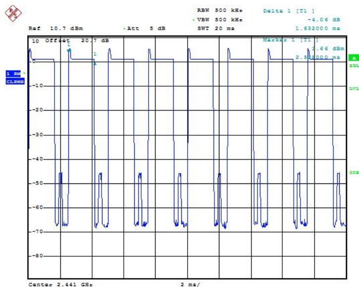
Fig.73 Number of Transmissions Measurement: Ch39, Packet 3-DH1
