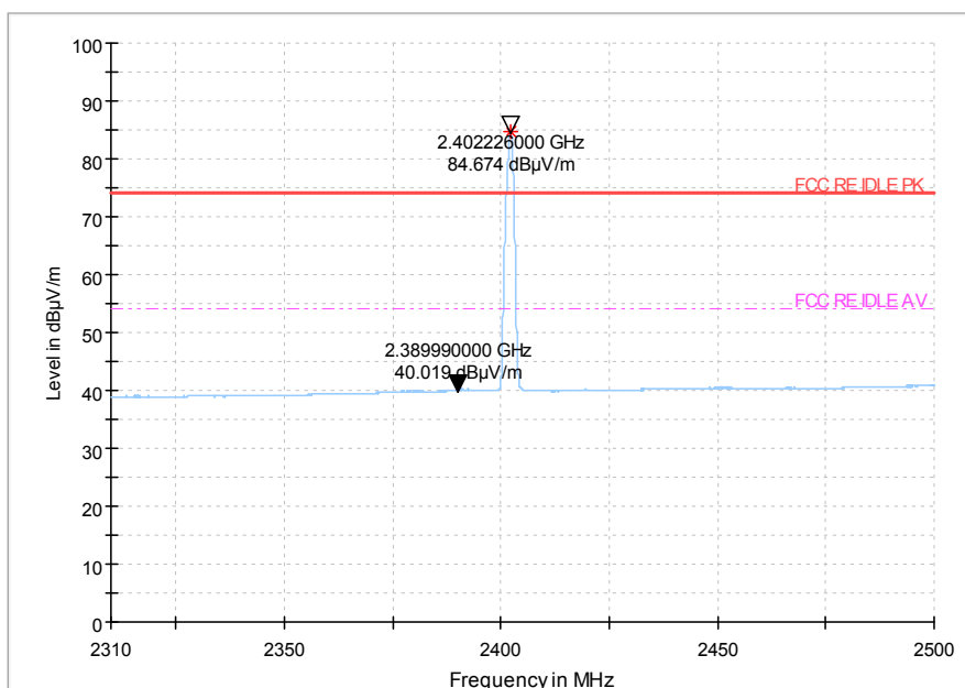
Fig.48 Radiated emission (Low): \pi/4 DQPSK, low channel
