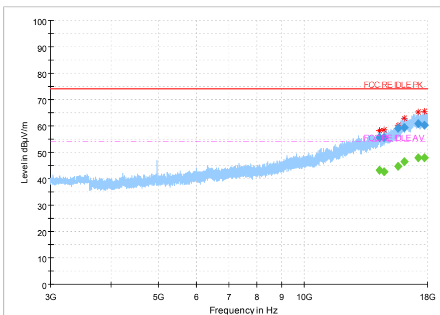
Fig.47 Radiated emission: \pi/4 DQPSK, Ch78, 3GHz~18GHz
