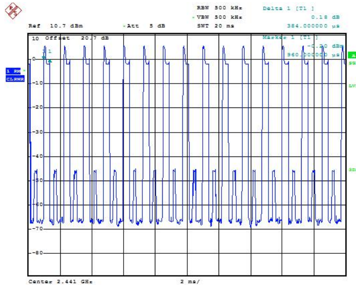
Fig.65 Number of Transmissions Measurement: Ch39, Packet DH5
