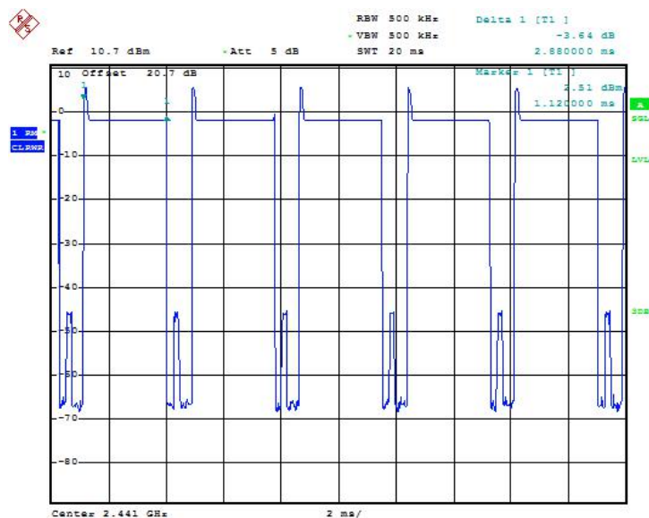
Fig.69 Number of Transmissions Measurement: Ch39, Packet 2-DH3
