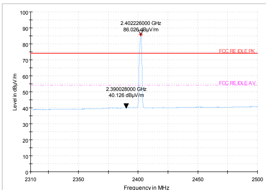
Fig.58 Radiated emission (Low): \pi/4 DQPSK, low channel
