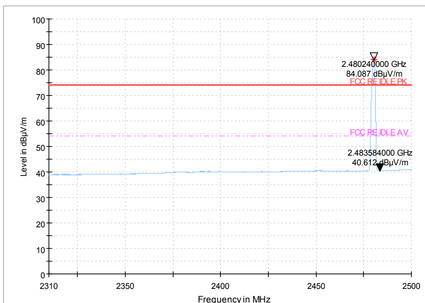
Fig.59 Radiated emission (High): \pi/4 DQPSK, high channel
