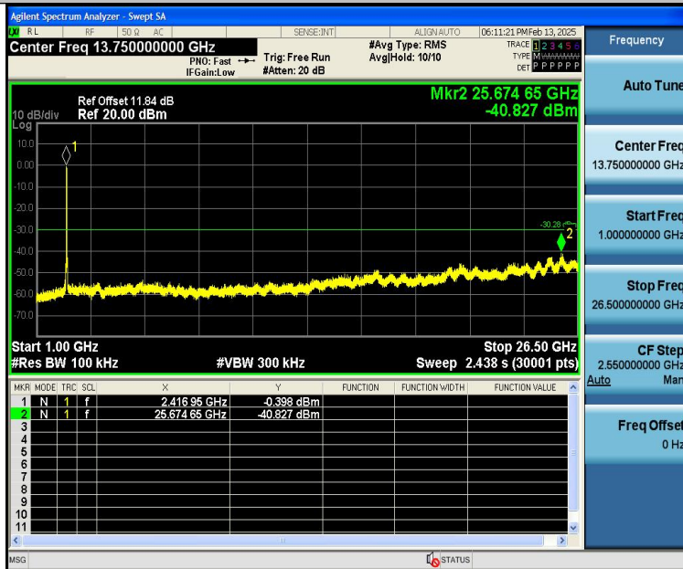
11N40SISO-Ant1-2437-0~Reference-PASS
