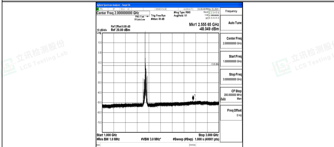
Band4_20MHz_QPSK_20300_1RB#0_1000~3000_1000~3000
