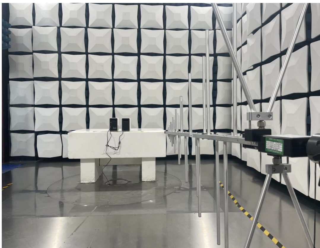
Photograph 2: Set-up for Radiated Spurious Emission, 30MHz - 1GHz
