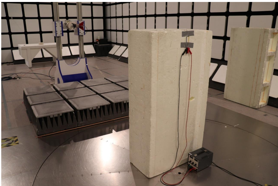
Photograph 5. Radiated emissions 1164 – 1240 MHz, 1559 – 1610 MHz, 1610 – 3500 MHz, and 4.5 – 10.6 GHz
