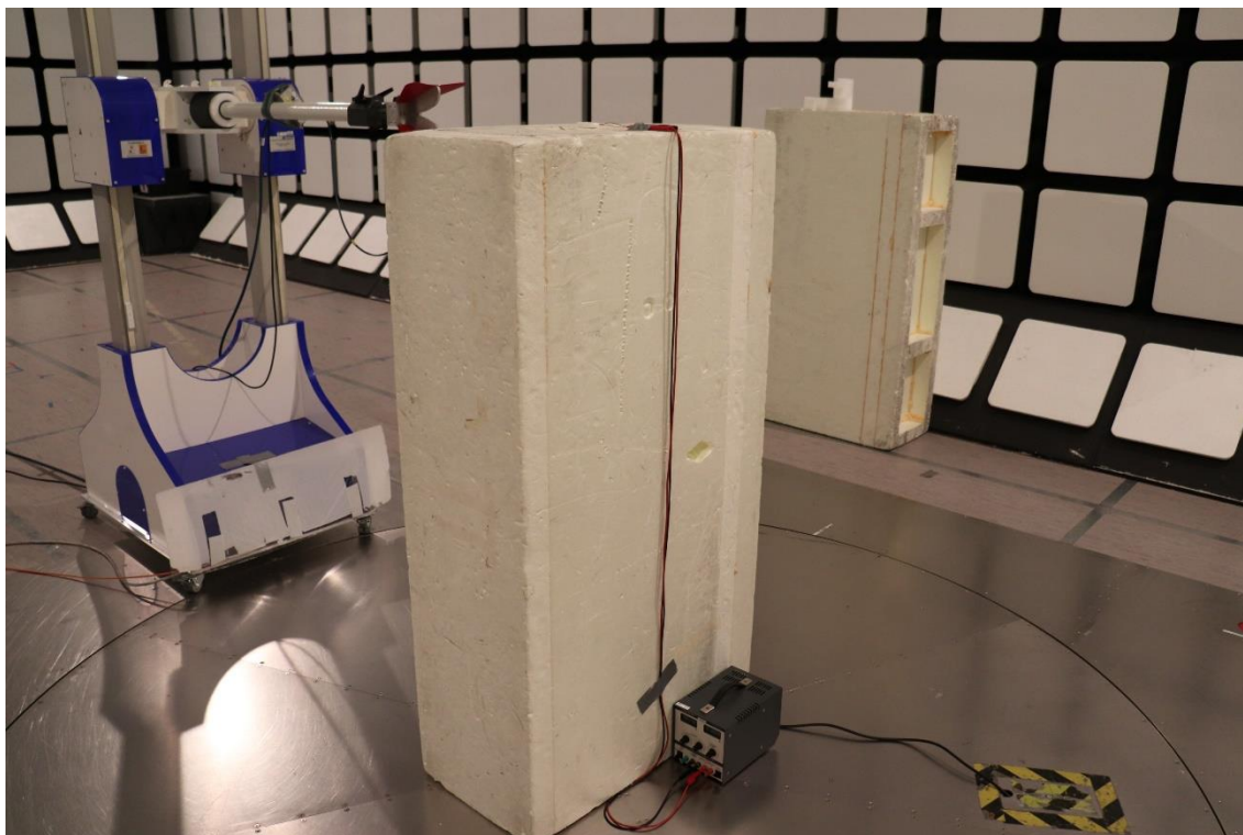
Photograph 4. Radiated emissions 1000 – 1610 MHz and 10.6 – 18 GHz
