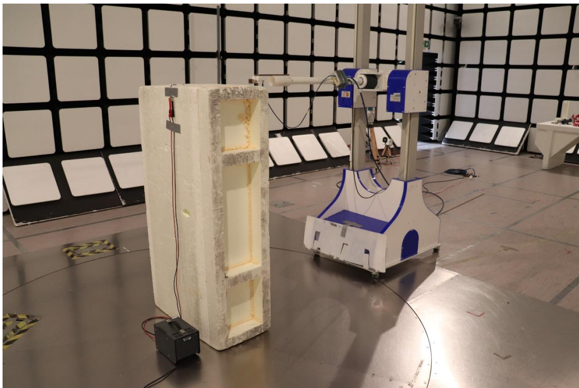
Photograph 6. Radiated emissions 18 – 26.5 GHz
