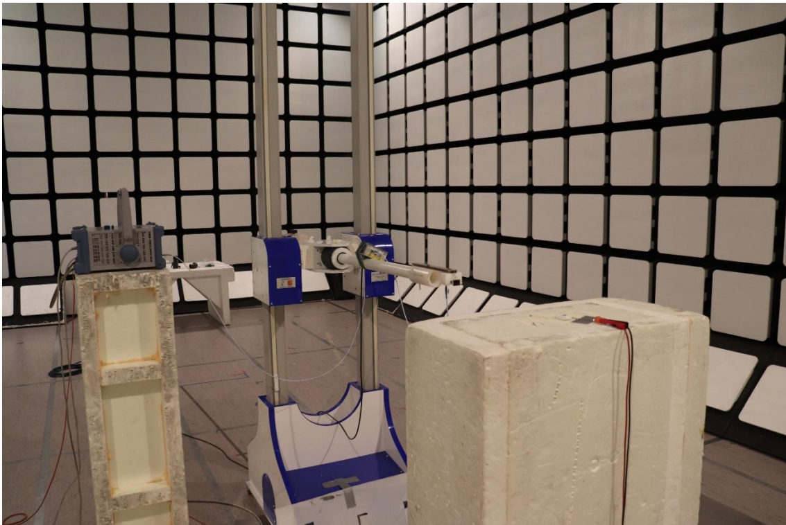
Photograph 7. Radiated emissions 26.5 – 40 GHz
