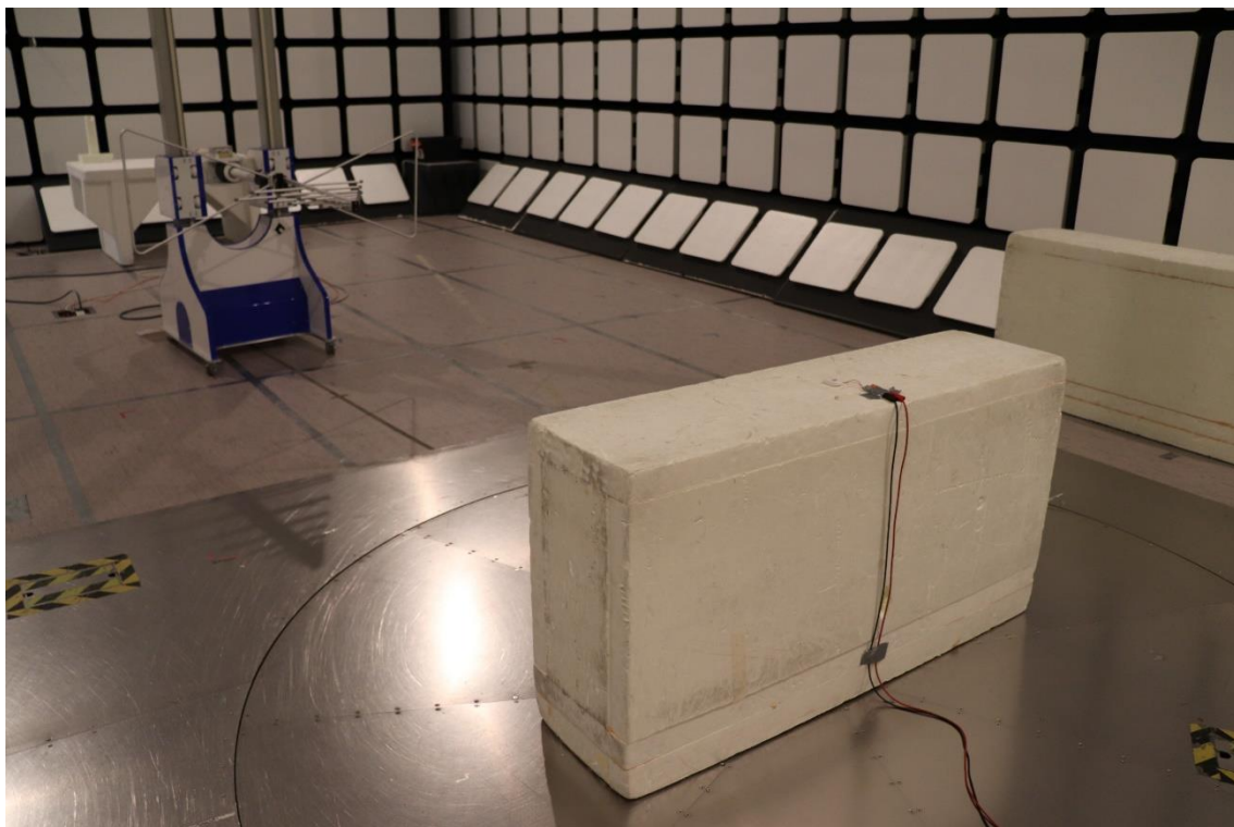
Photograph 2. Radiated emissions 30 – 960 MHz
