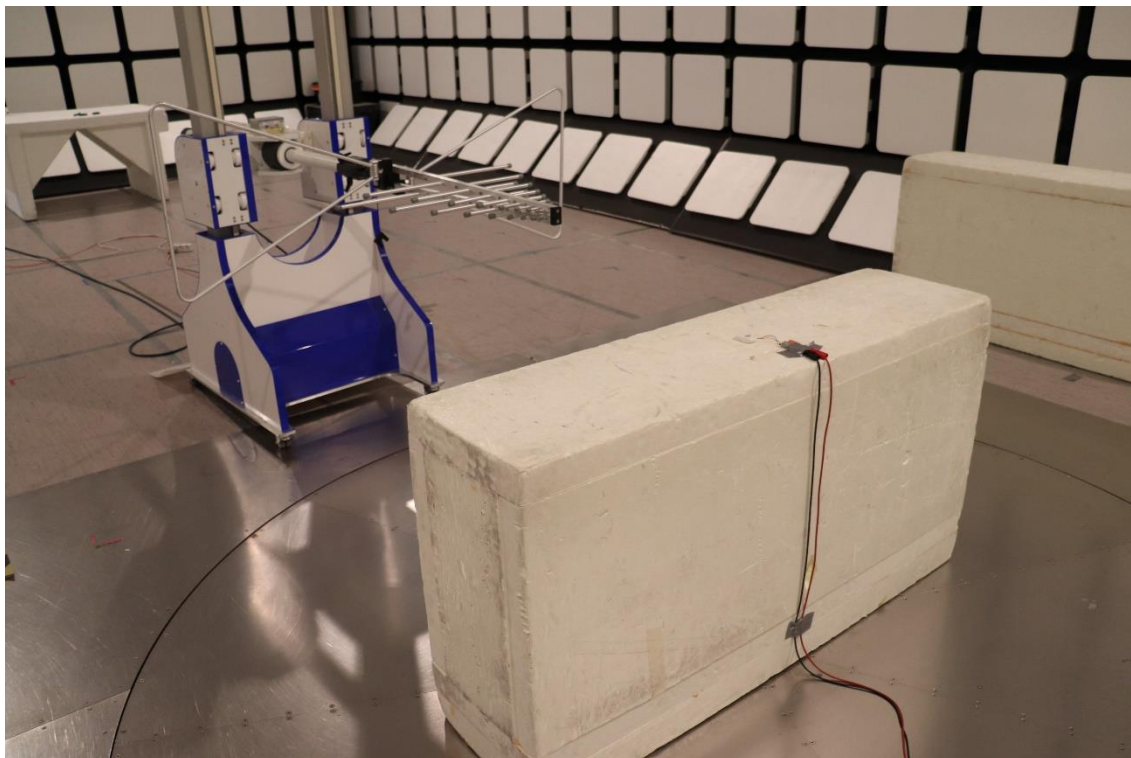
Photograph 3. Radiated emissions 960 – 1000 MHz
