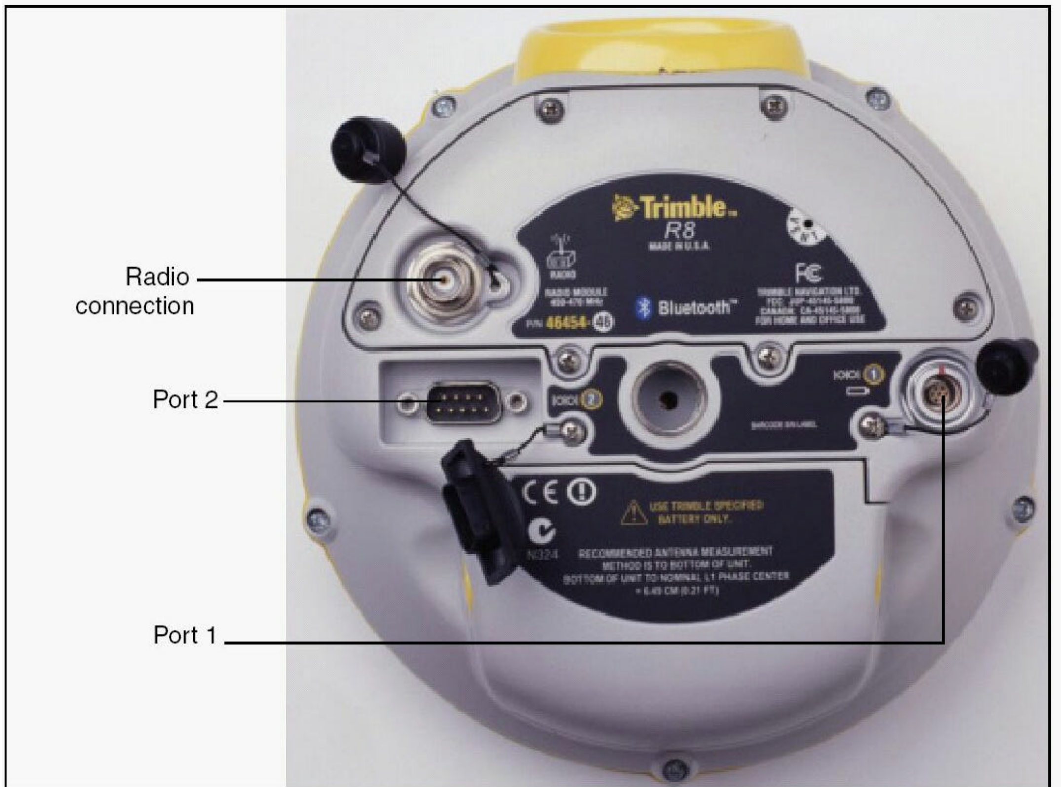
Figure 13.2 Trimble R8 lower housing
