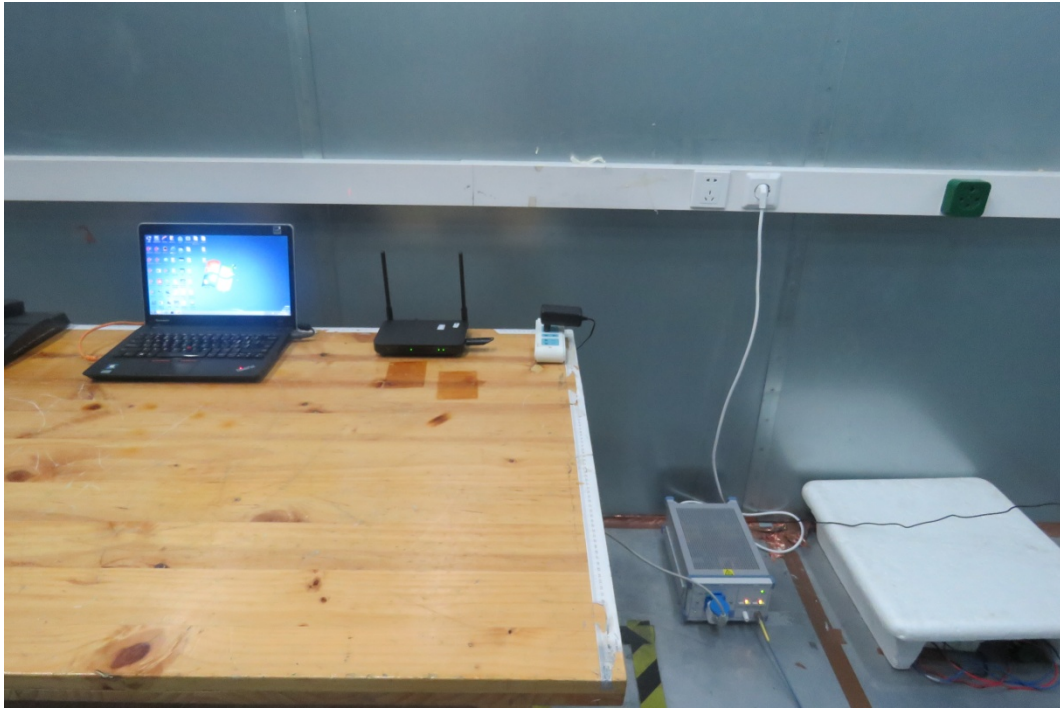
Conducted Emission Test Setup
