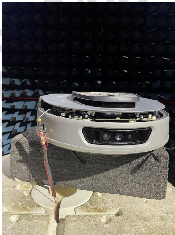
The coordinate system of Chamber/暗室坐标系
