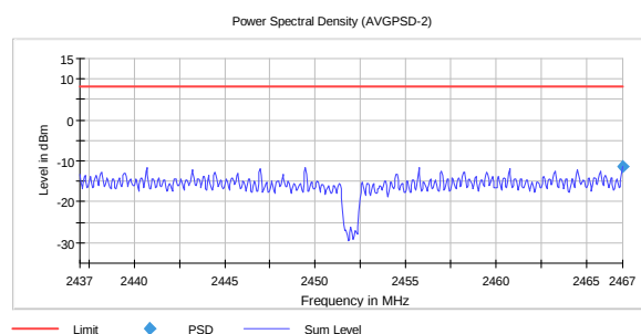
PSD, 2452 MHz, 802.11n HT40 SISO MCS7 -11.5
