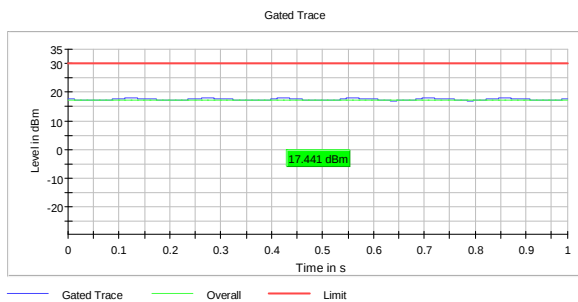
RMS Power, 2457 MHz, 802.11b 1M
