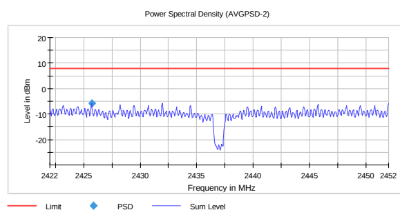
PSD, 2437 MHz, 802.11n HT40 MIMO MCS15 -5.9
