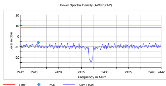
PSD, 2427 MHz, 802.11n HT40 MIMO MCS15 -6.1
