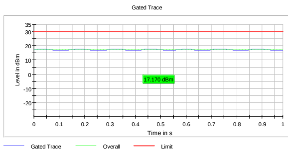
RMS Power, 2417 MHz, 802.11b 1M
