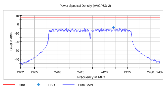
PSD, 2417 MHz, 802.11n MIMO MCS15 -3.78
