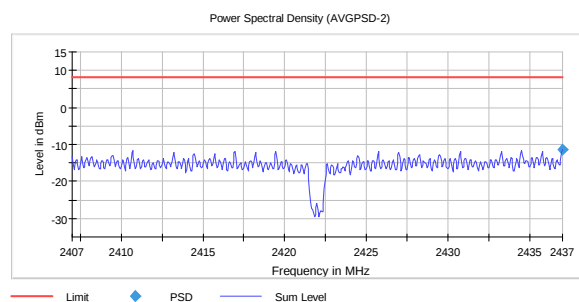
PSD, 2422 MHz, 802.11n HT40 MIMO MCS15 -11.5
