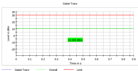
RMS Power, 2452 MHz, 802.11n HT40 MIMO MCS8
