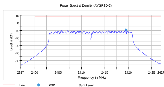
PSD, 2412 MHz, 802.11n MIMO MCS15 -9.17
