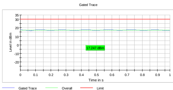
RMS Power, 2437 MHz, 802.11b 1M
