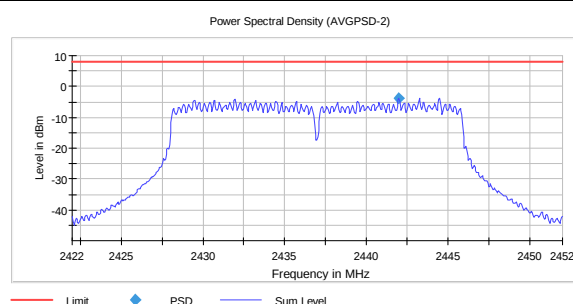
PSD, 2437 MHz, 802.11n MIMO MCS15 -3.69
