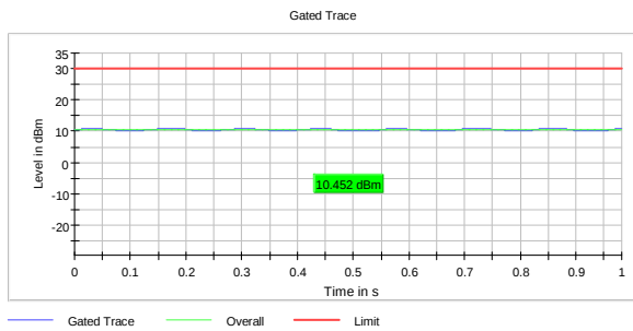
RMS Power, 2412 MHz, 802.11b 1M
