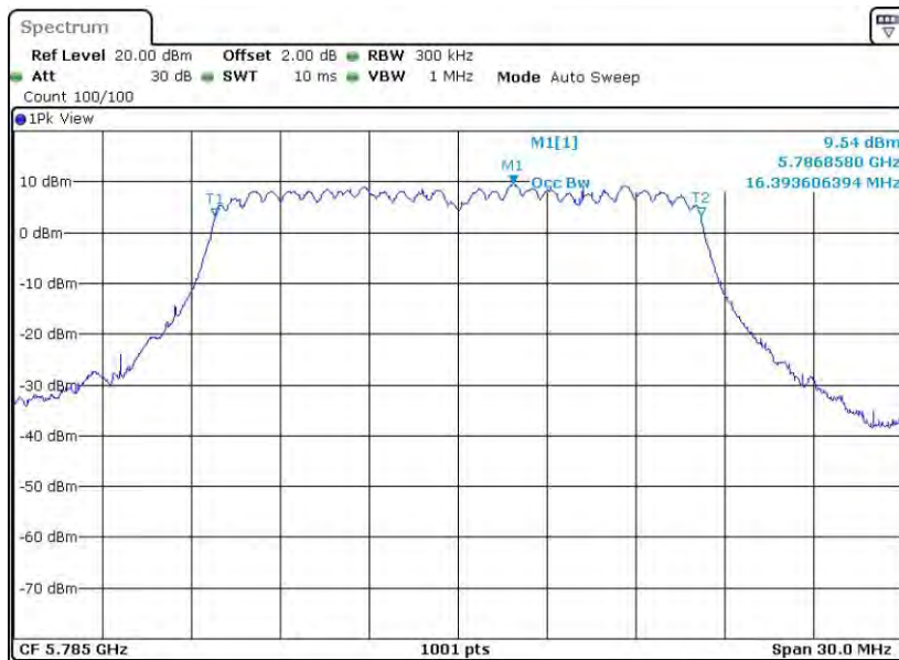
11A-CDD_Ant2_5785
