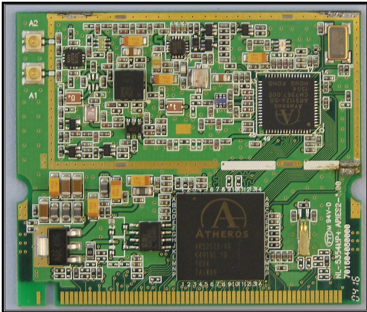
PHOTOGRAPH 14: 802.11G WLAN TOP VIEW UNSHIELDED
