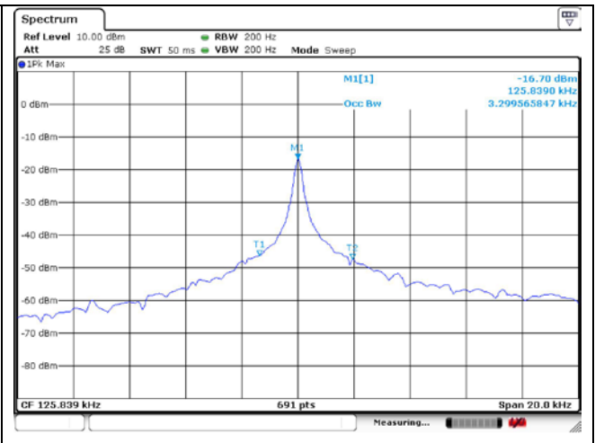
INT1 Antenna
