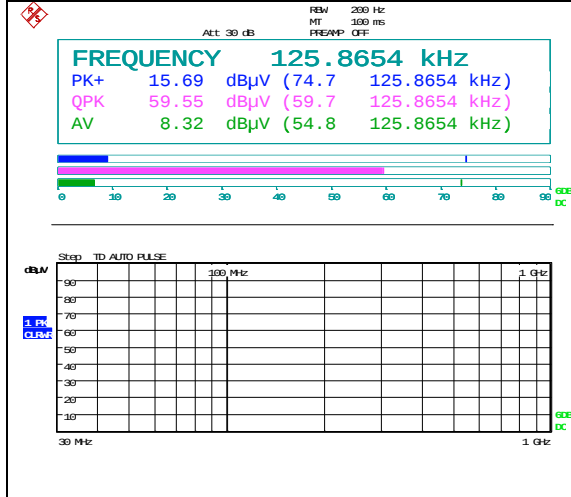
DRV Antenna
