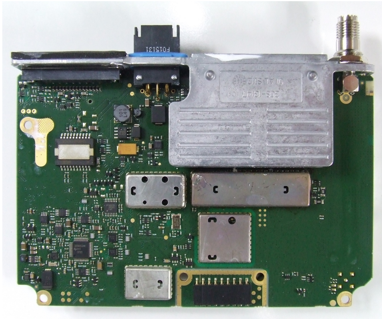
Photograph 03: Radio - Main PCB bottom with shields
