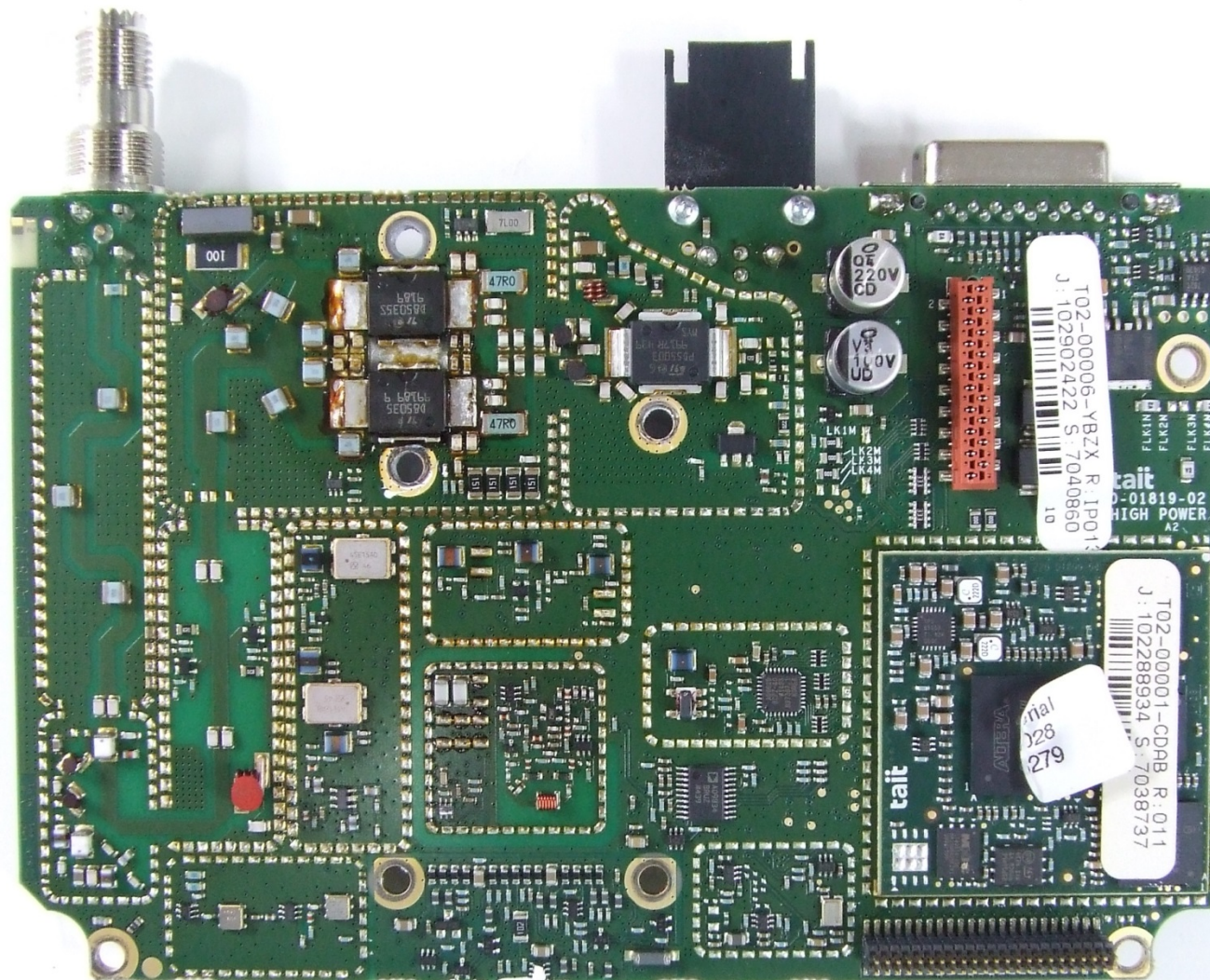
Photograph 02: Radio - Main PCB top without shields
