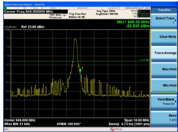
eMTC Band 5 16QAM 5MHz CH-High 100%RB
