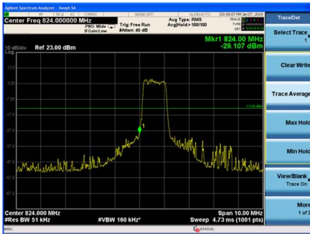
eMTC Band 5 16QAM 3MHz CH-Low 1RB
