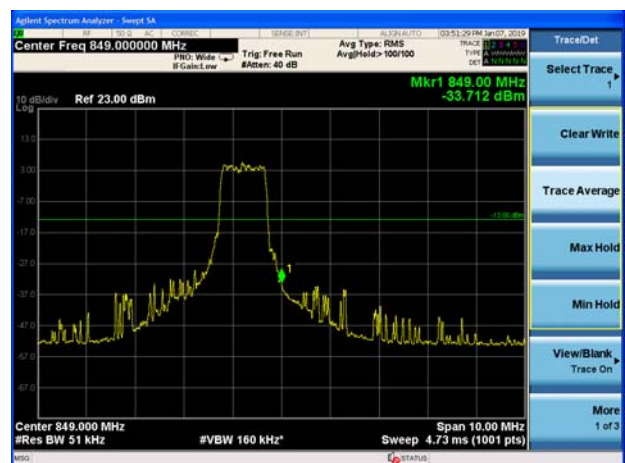
eMTC Band 5 16QAM 3MHz CH-High 100%RB
