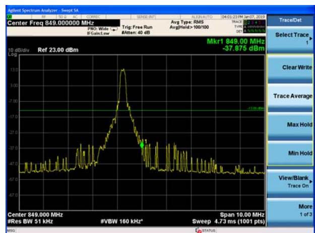
eMTC Band 5 16QAM 10MHz CH-High 1RB
