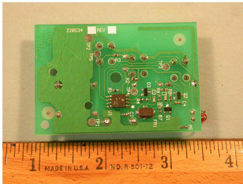
PCB Assembly, Front and Back View, MT-3 Transmitter
