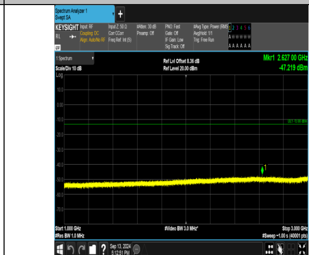
Band26_3MHz_QPSK_26740_15RB#0_1000~3000_1000~3000
