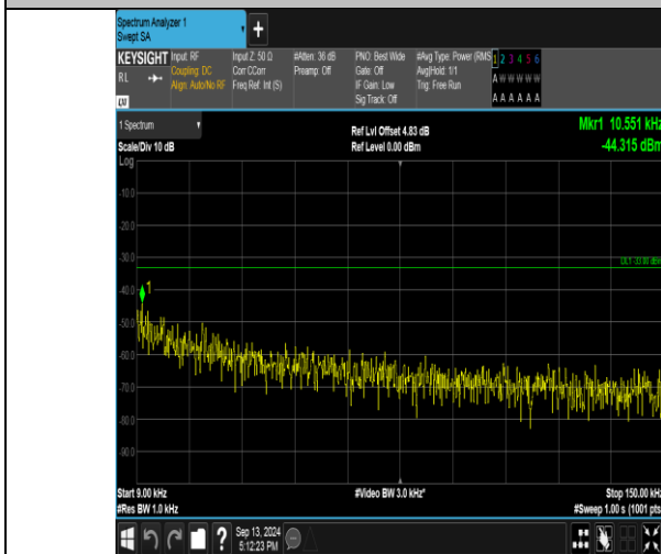
Band26_3MHz_QPSK_26740_15RB#0_0.009~0.15_0.009~0.15
