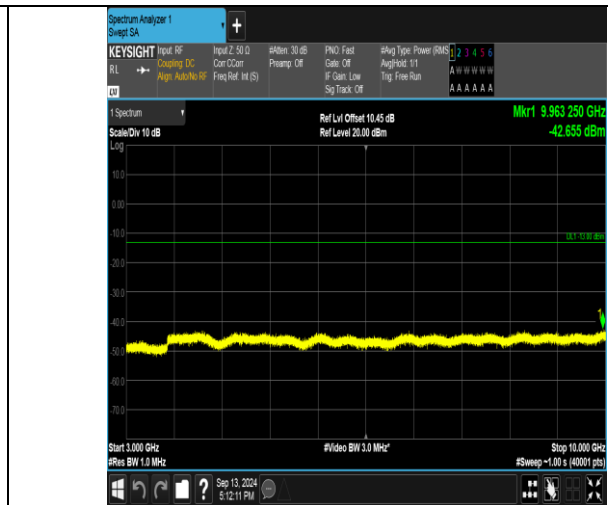
Band26_3MHz_16QAM_26740_1RB#14_3000~10000_3000~10000
