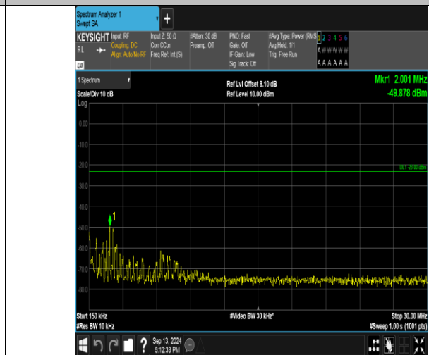
Band26_3MHz_QPSK_26740_15RB#0_0.15~30_0.15~30
