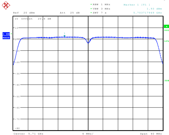
Figure 7-37: Peak Power Spectral Density 802.11ac, Channel 142, MCS0 Mbps
