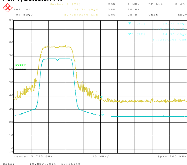
Figure 3-15: Band-Edge Compliance of RF Radiated Emission. 802.11n, Ch. 140, 5700 MHz, Centre of Band-Edge: 5725 MHz Pol: V, Detector: PK
