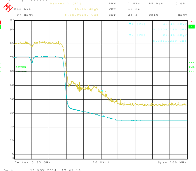
Figure 3-20: Band-Edge Compliance of RF Radiated Emission. 802.11n, Ch. 62, 5310 MHz, Centre of Band-Edge: 5350 MHz Pol: H, Detector: PK
