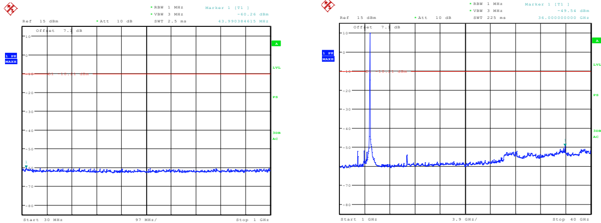
Figure 7-49a: Spurious RF Conducted Emissions, 802.11ac Channel 142, MCS0
