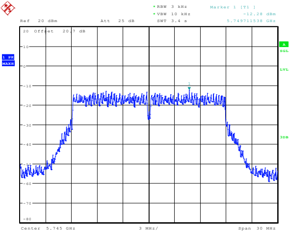
Figure 7-34: Peak Power Spectral Density 802.11ac, Channel 149, MCS0 Mbps
