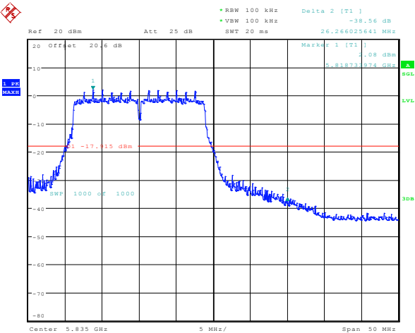
Figure 7-18: Band Edge Compliance 802.11ac, Channel 165, MCS0 Mbps
