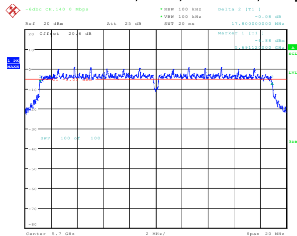
Figure 7-3: 6 dB Bandwidth
