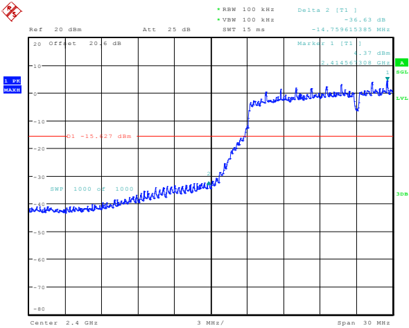
Figure 5-14: Band Edge Compliance 802.11n, Channel 1, MCS 0
