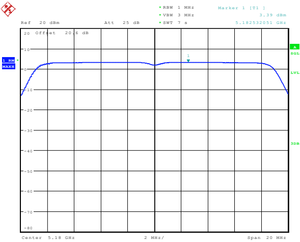
Figure 6-28: Peak Power Spectral Density 802.11n, Channel 36, MCS 0
