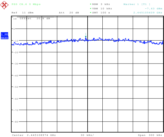
Figure 5-23: Peak Power Spectral Density 802.11n, Channel 6, MCS 0
