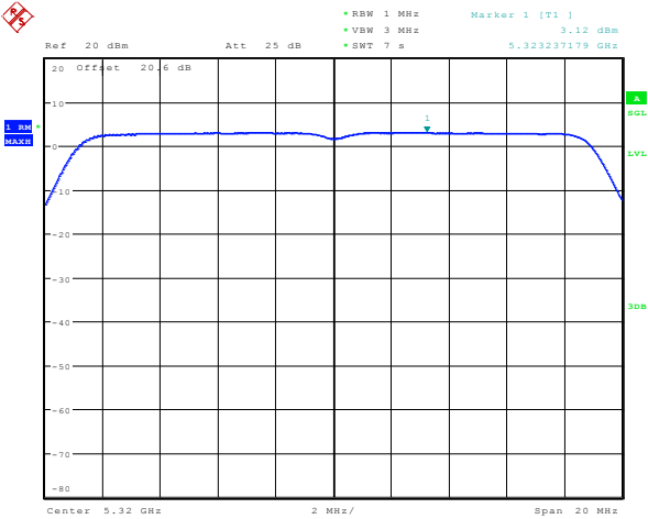
Figure 7-32: Peak Power Spectral Density 802.11ac, Channel 64, MCS0 Mbps
