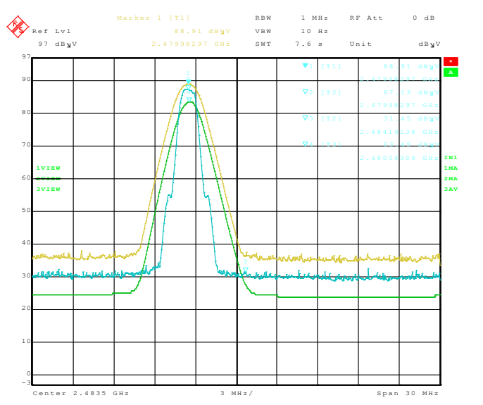
Figure 2-12: Band-Edge Compliance of RF Rad. Emissions.
