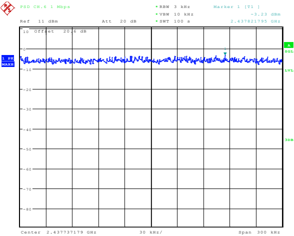
Figure 5-17: Peak Power Spectral Density 802.11b, Channel 6, 1 Mbps
