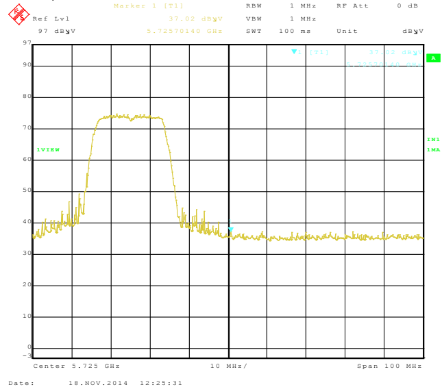
Figure 4-8: Band-Edge Compliance of RF Radiated Emission. 802.11ac, Ch. 140, 5700 MHz, Centre of Band-Edge: 5725 MHz Pol: H, Detector: PK
