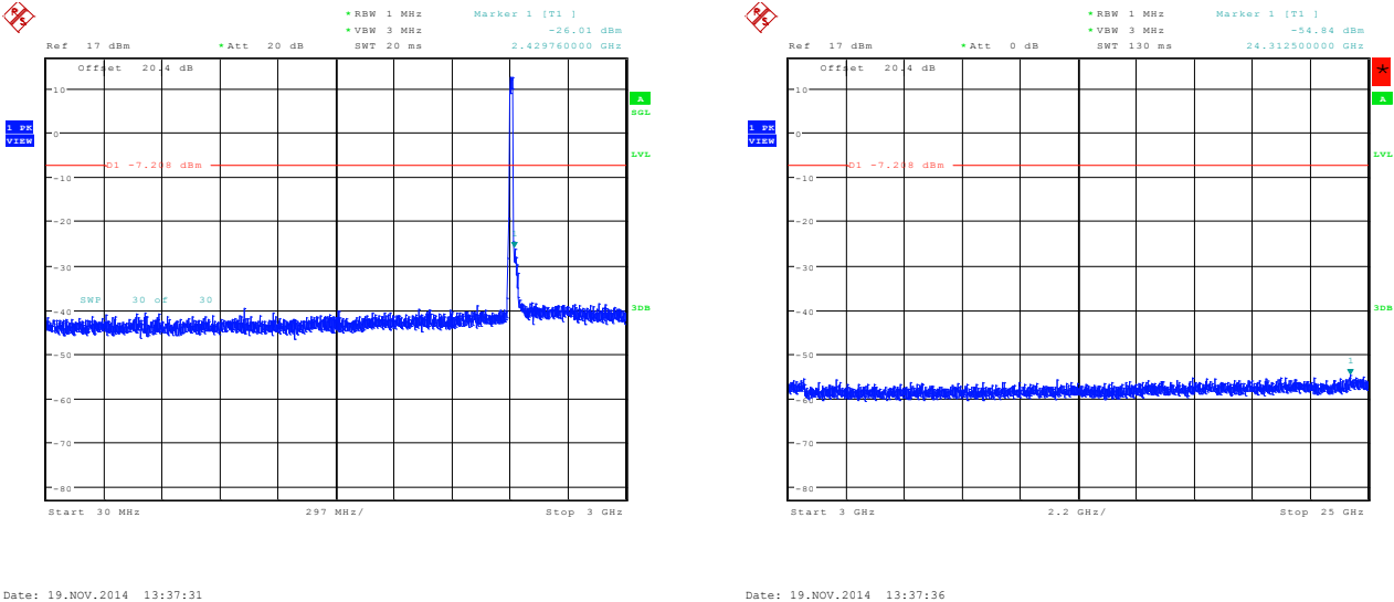
Figure 5-31: Spurious Conducted RF Emissions 802.11n, Channel 1, MCS 0
