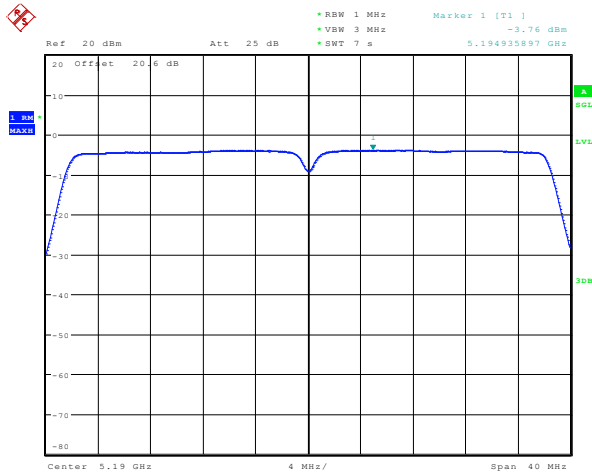
Figure 7-35: Peak Power Spectral Density 802.11ac, Channel 38, MCS0 Mbps
