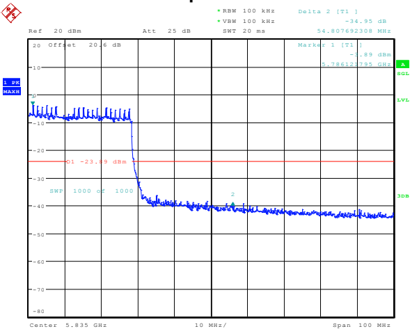
Figure 7-30: Band Edge Compliance 802.11ac, Channel 155 ( high edge ), MCS0 Mbps
