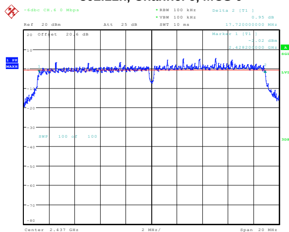
Figure 5-8: 6 dB Bandwidth 802.11n, Channel 6, MCS 0
