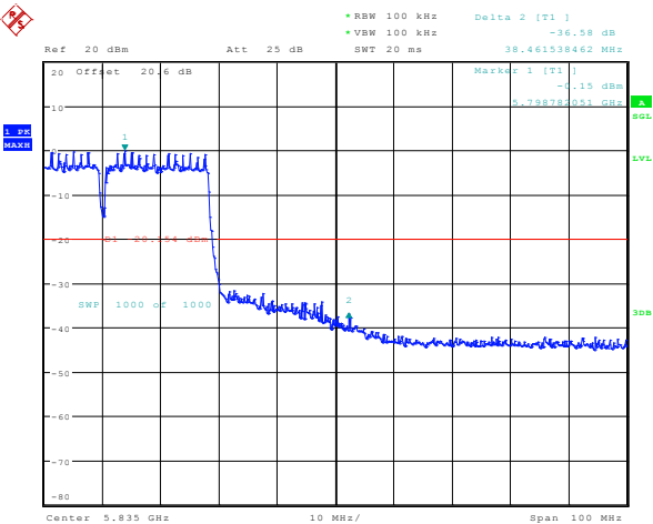
Figure 7-24: Band Edge Compliance 802.11ac, Channel 159, MCS0 Mbps
