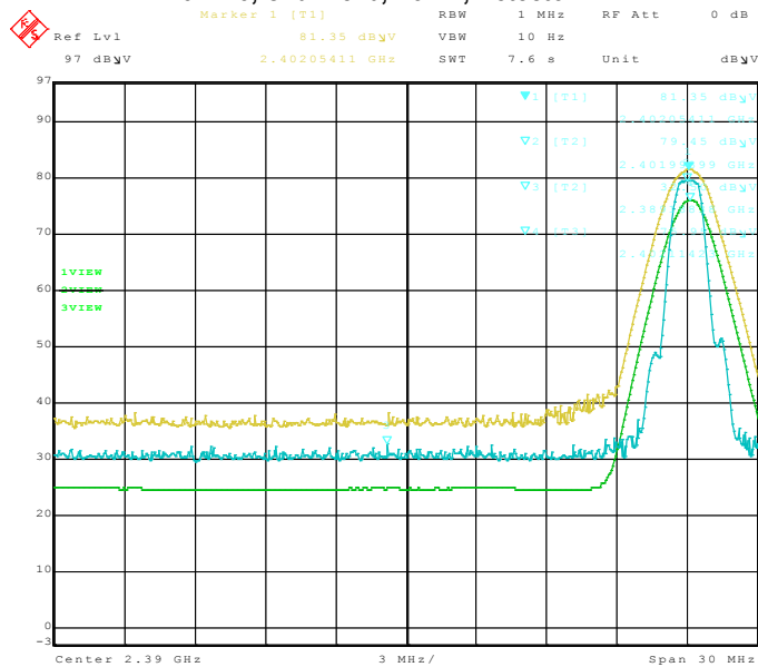
Figure 2-11: Band-Edge Compliance of RF Rad. Emissions.
