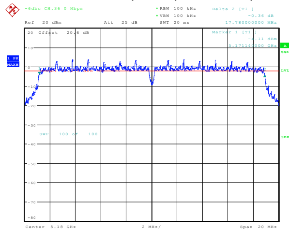
Figure 7-1: 6 dB Bandwidth
