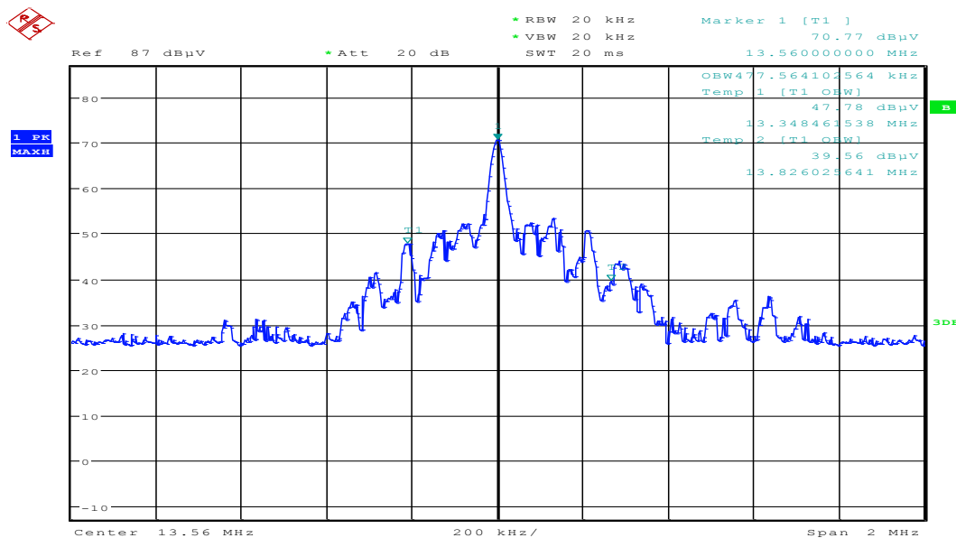
Figure 8-1: Occupied Bandwidth, NFC TX Frequency = 13.56 MHz
