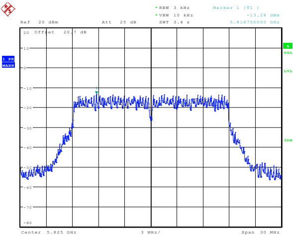
Figure 6-30: Peak Power Spectral Density 802.11n, Channel 165, MCS 0
