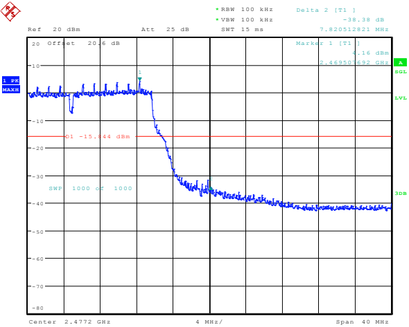
Figure 5-15: Band Edge Compliance 802.11n, Channel 11, MCS 0
