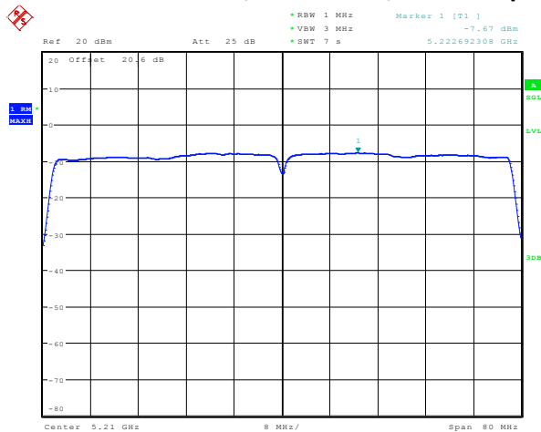
Figure 7-39: Peak Power Spectral Density 802.11ac, Channel 42, MCS0 Mbps
