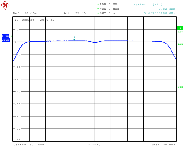
Figure 7-33: Peak Power Spectral Density 802.11ac, Channel 140, MCS0 Mbps
