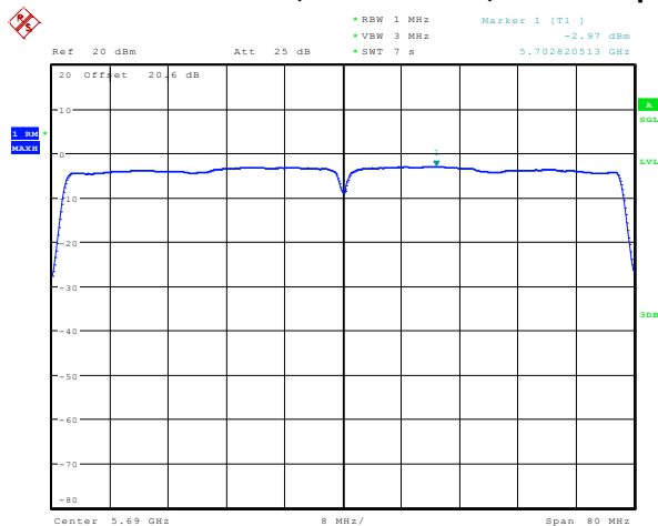
Figure 7-41: Peak Power Spectral Density 802.11ac, Channel 138, MCS0 Mbps
