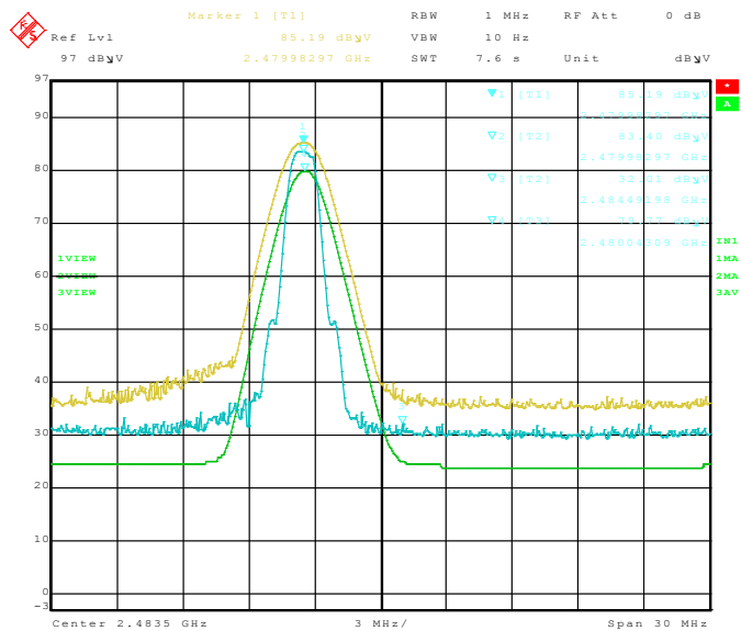
Figure 2-11: Band-Edge Compliance of RF Rad. Emissions.
