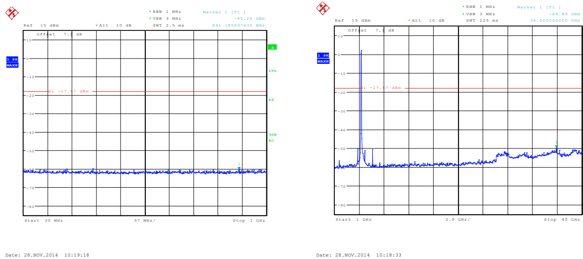
Figure 7-52a: Spurious RF Conducted Emissions, 802.11ac Channel 58, MCS0
