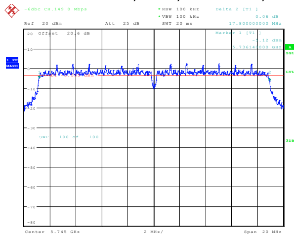
Figure 7-4: 6 dB Bandwidth
