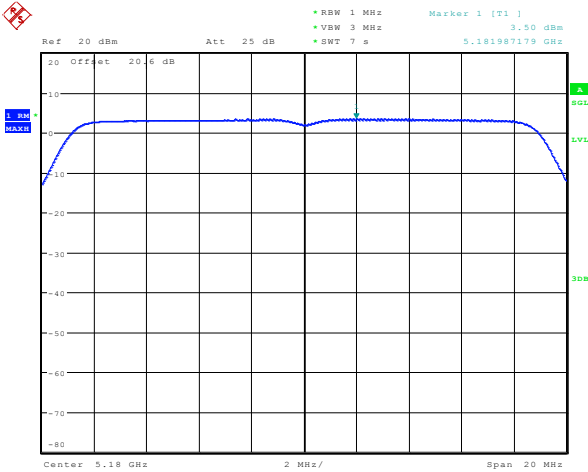
Figure 7-31: Peak Power Spectral Density 802.11ac, Channel 36, MCS0 Mbps
