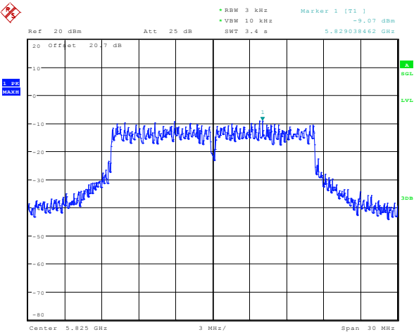
Figure 6-27: Peak Power Spectral Density 802.11a, Channel 165, 6 Mbps
