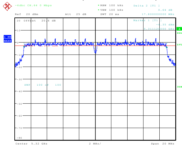
Figure 7-2: 6 dB Bandwidth
