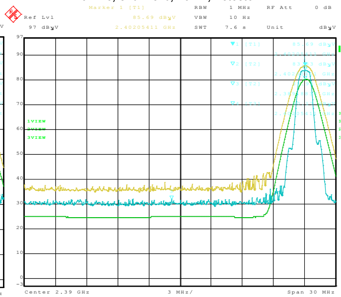
Figure 2-12: Band-Edge Compliance of RF Rad. Emissions.
