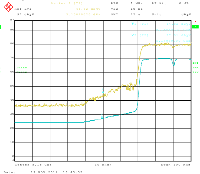
Figure 3-18: Band-Edge Compliance of RF Radiated Emission. 802.11n, Ch. 38, 5190 MHz, Centre of Band-Edge: 5150 MHz Pol: H, Detector: PK
