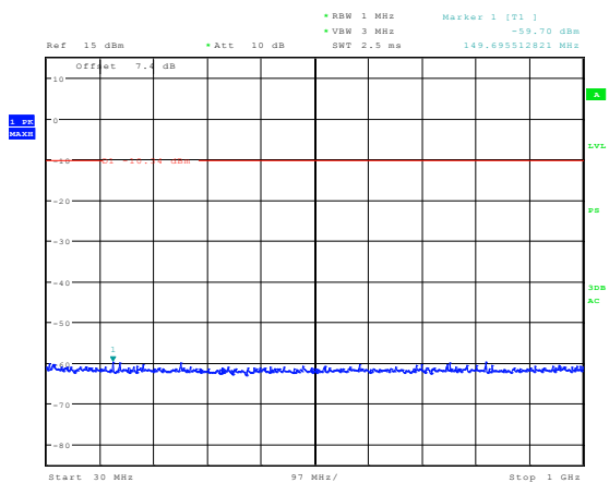
Figure 6-34a: Spurious RF Conducted Emissions, 802.11a Channel 140, 6 Mbps
