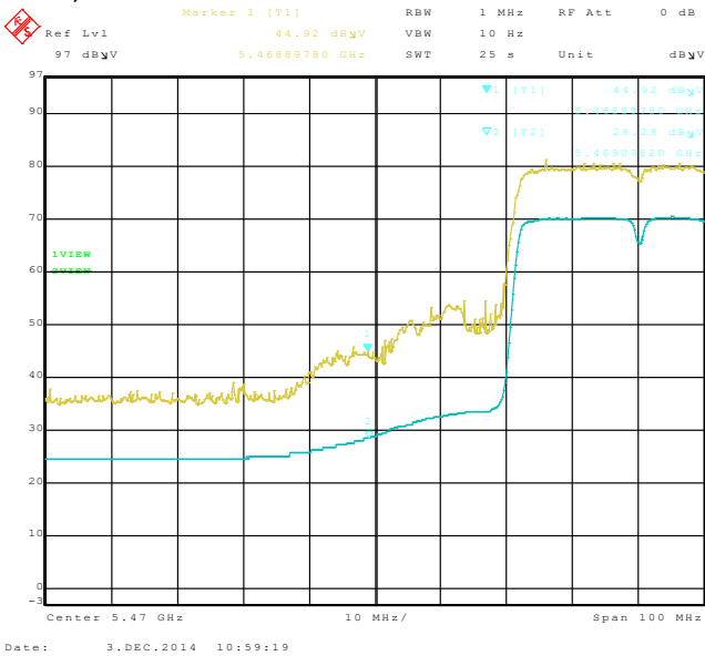
Figure 3-21: Band-Edge Compliance of RF Radiated Emission 802.11n, Ch. 102, 5510 MHz, Centre of Band-Edge: 5470 MHz Pol: V, Detector: PK
