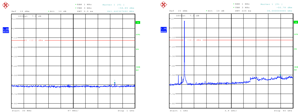
Figure 7-50a: Spurious RF Conducted Emissions, 802.11ac Channel 151, MCS0
