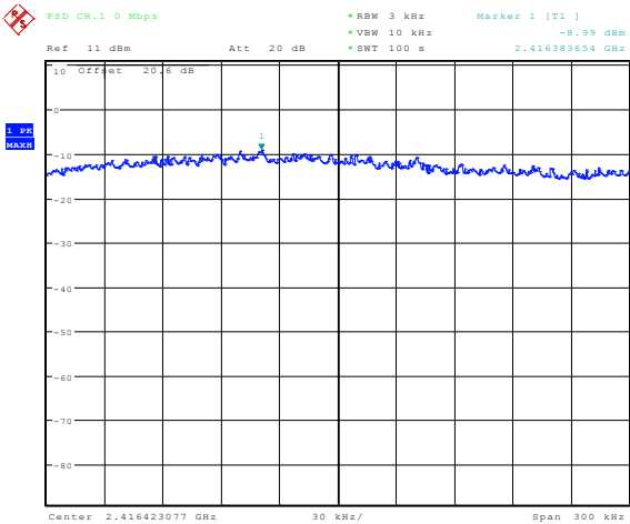
Figure 5-22: Peak Power Spectral Density 802.11n, Channel 1, MCS 0
