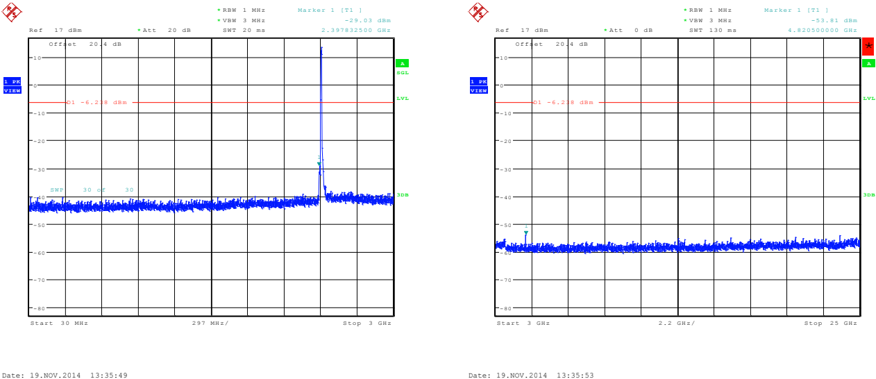
Figure 5-25: Spurious Conducted RF Emissions 802.11b, Channel 1, 1 Mbps
