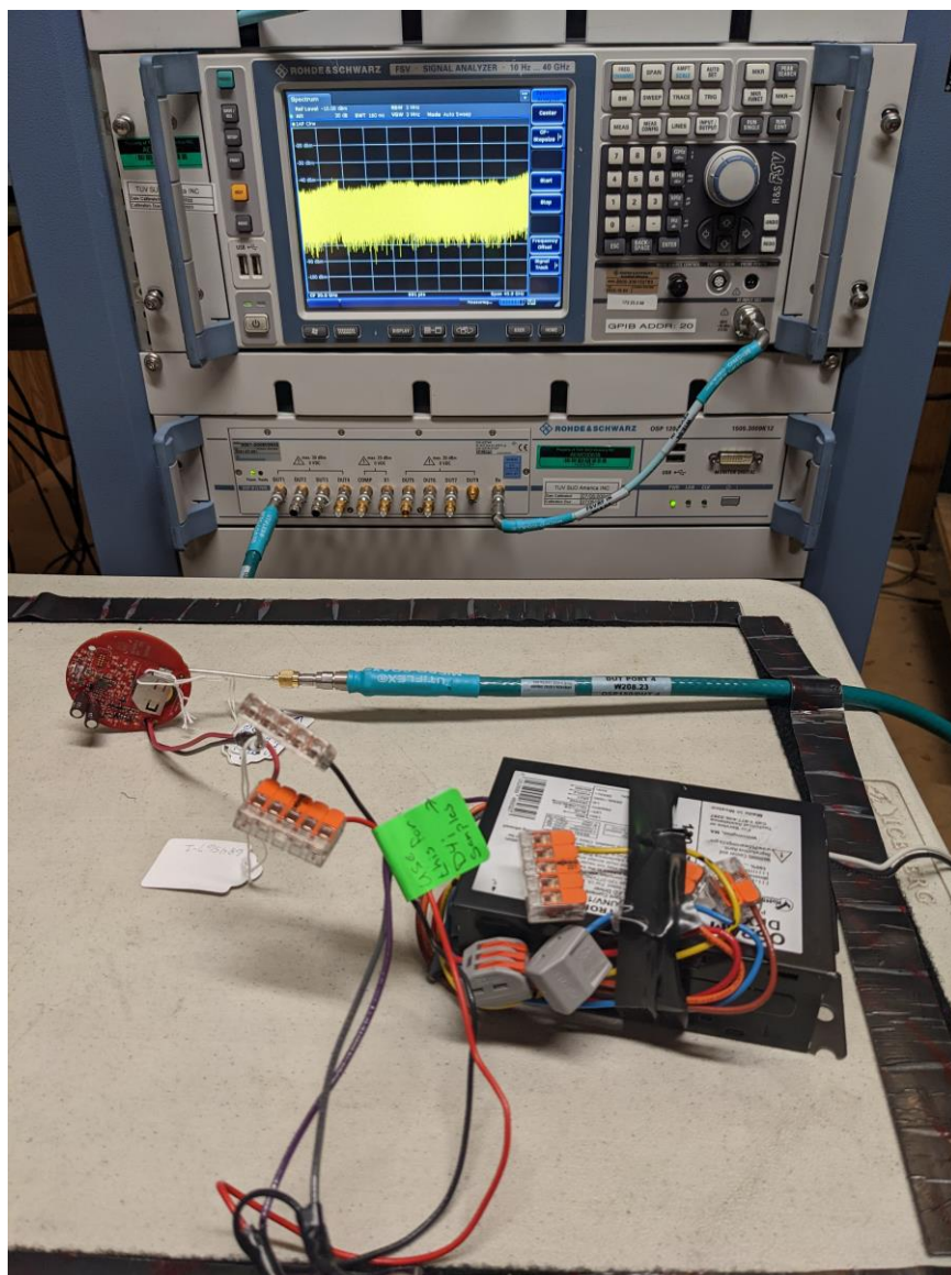
Figure 7: Test Setup – Antenna Port Measurement
