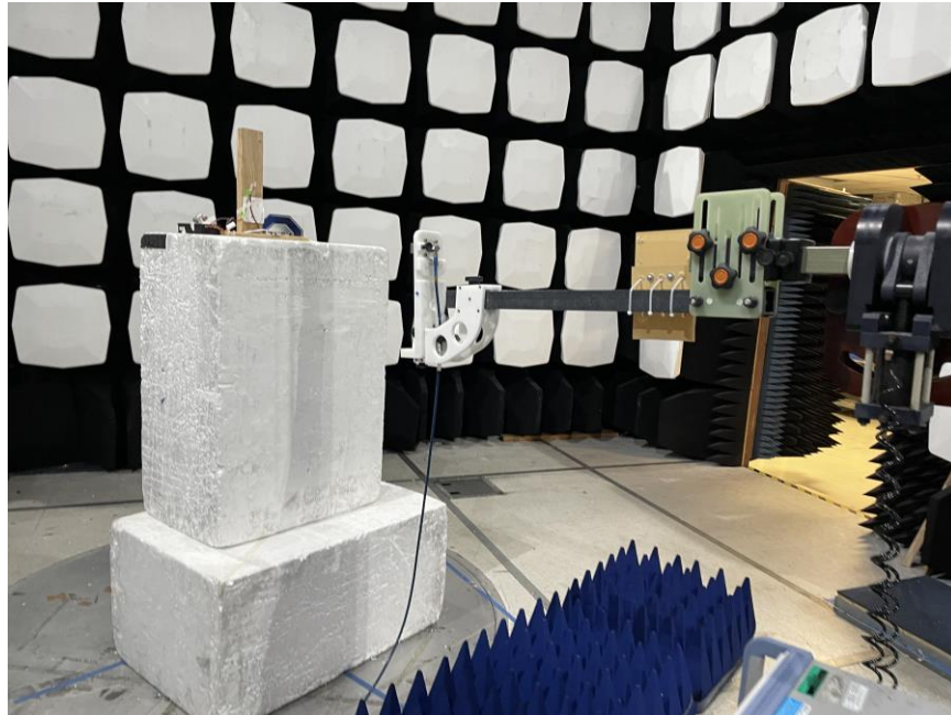
Figure 5: Test Setup – Radiated Emissions >18GHz
