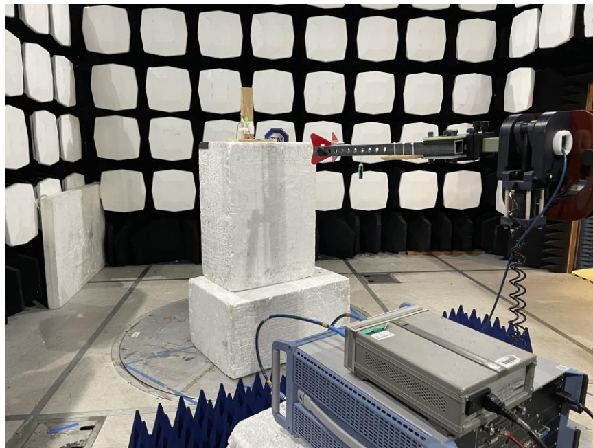
Figure 4: Test Setup – Radiated Emissions >10GHz
