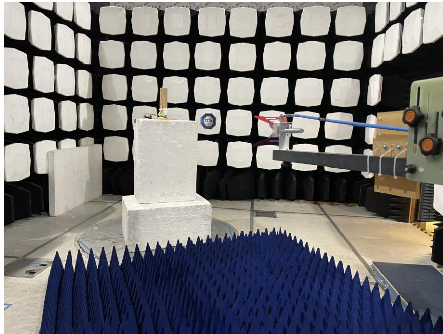
Figure 3: Test Setup – Radiated Emissions >1GHz
