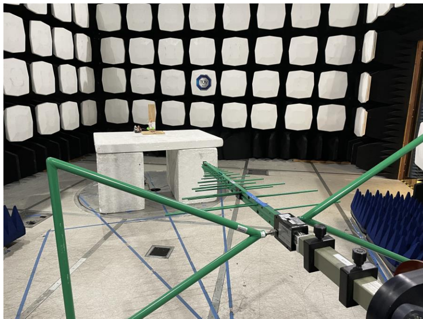
Figure 2: Test Setup – Radiated Emissions <1GHz
