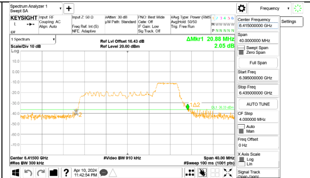
HIGH CHANNEL Antenna 4
