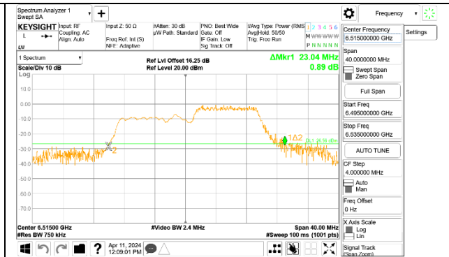
HIGH CHANNEL Antenna 3
