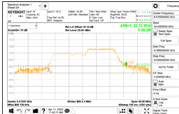
HIGH CHANNEL Antenna 1
