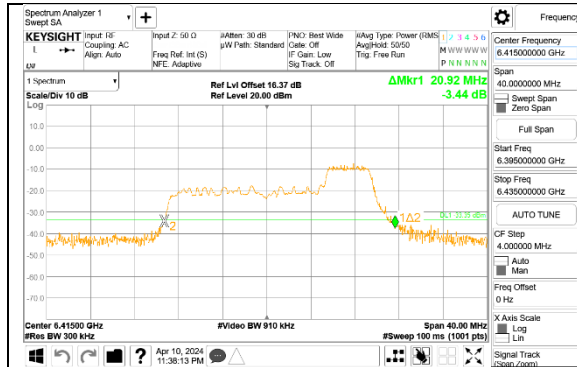
HIGH CHANNEL Antenna 2
