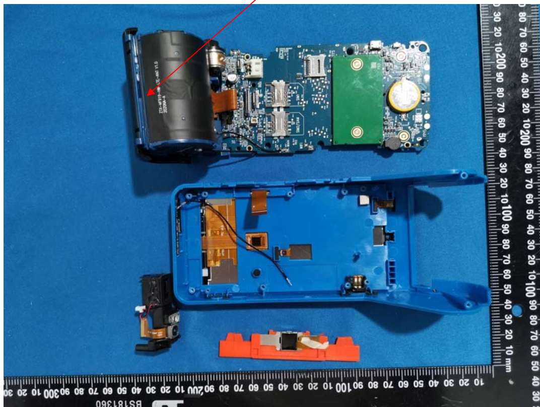
Wi-Fi/Bluetooth Antenna
