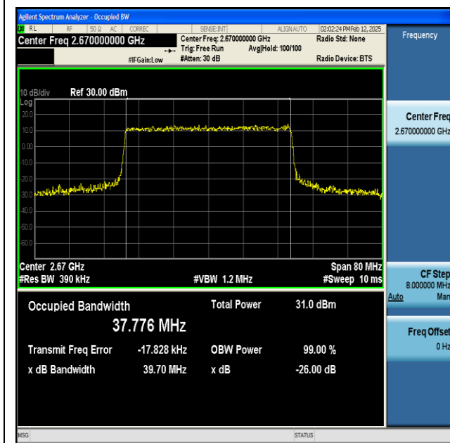
NTNV-n41-PC2-30-40-H-CP-16QAM-Outer_Full-Ant1-PASS
