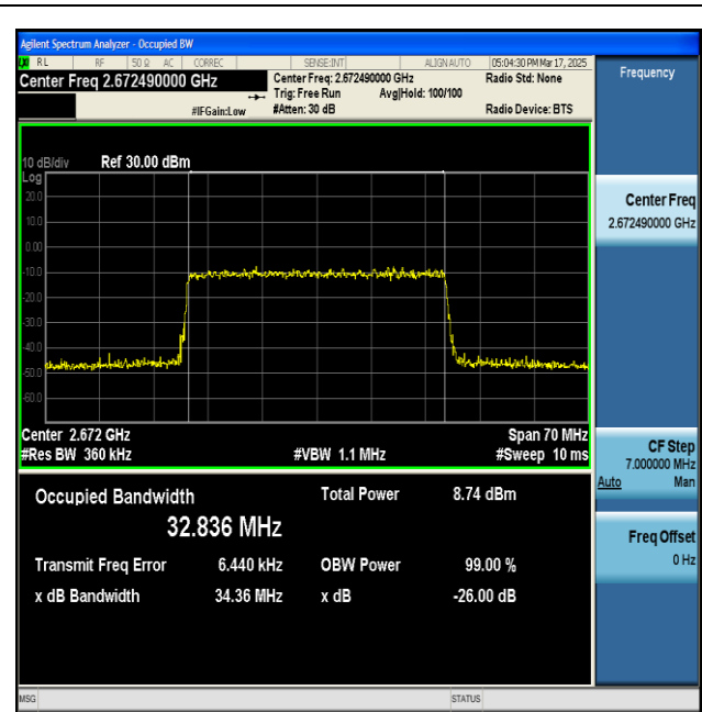
NTNV-n41-PC2-30-35-H-CP-256QAM-Outer_Full-Ant1- PASS
