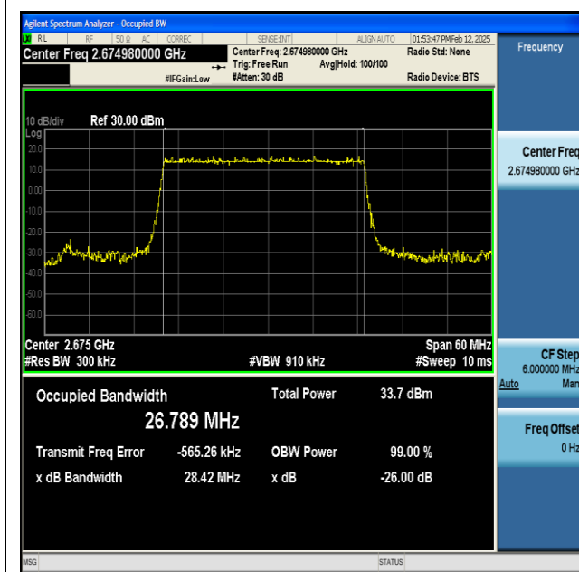
NTNV-n41-PC2-30-30-H-DFT-BPSK-Outer_Full-Ant1- PASS
