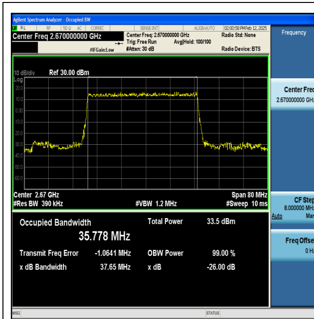
NTNV-n41-PC2-30-40-H-DFT-BPSK-Outer_Full-Ant1- PASS
