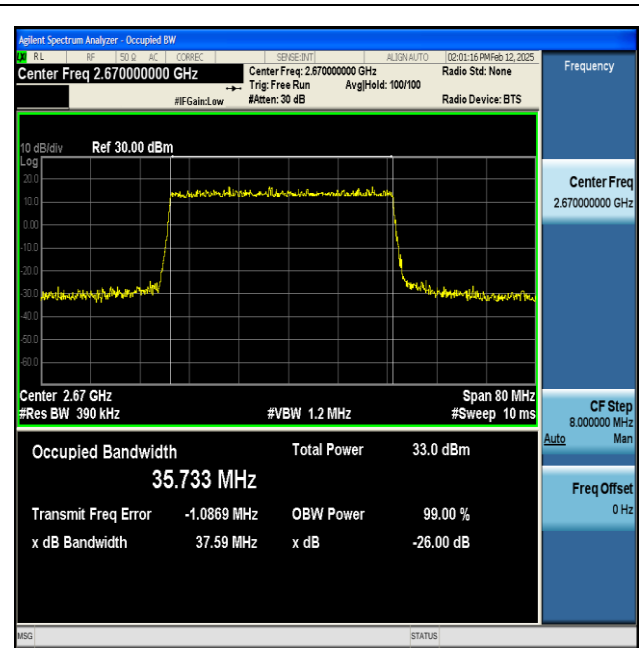
NTNV-n41-PC2-30-40-H-DFT-QPSK-Outer_Full-Ant1- PASS
