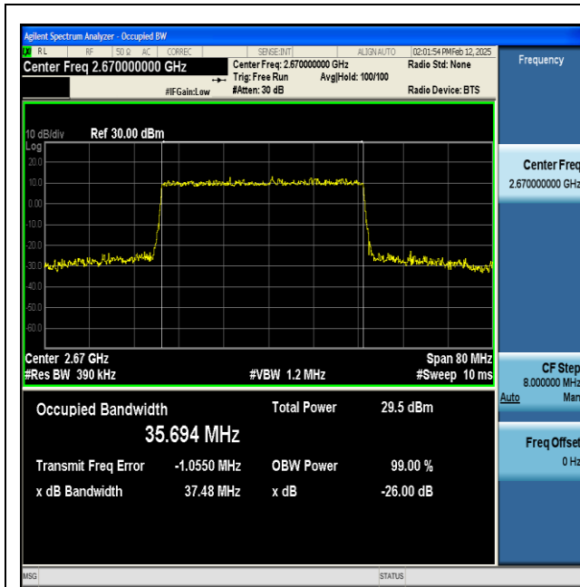
NTNV-n41-PC2-30-40-H-DFT-256QAM-Outer_Full-Ant1-PASS
