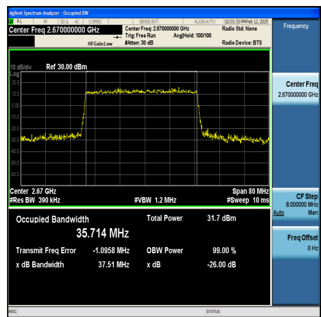
NTNV-n41-PC2-30-40-H-DFT-64QAM-Outer_Full-Ant1- PASS
