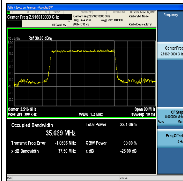
NTNV-n41-PC2-30-40-L-DFT-BPSK-Outer_Full-Ant1- PASS
