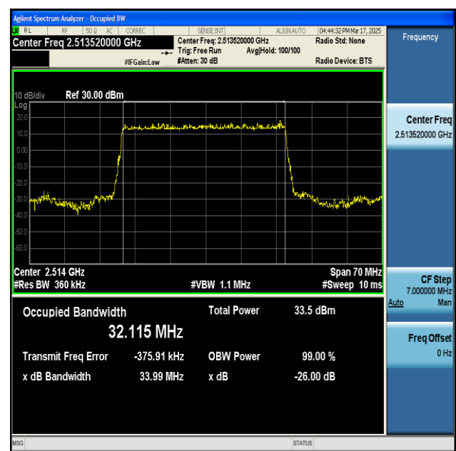
NTNV-n41-PC2-30-35-L-DFT-BPSK-Outer_Full-Ant1- PASS
