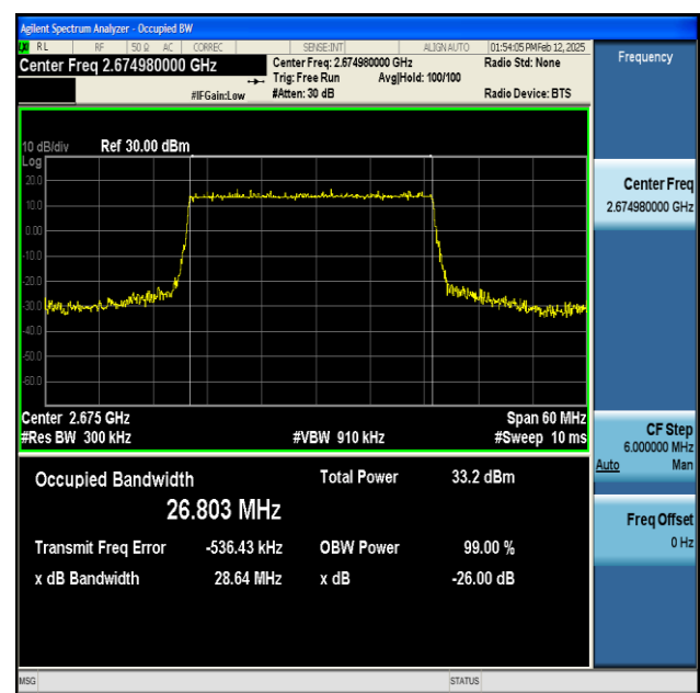
NTNV-n41-PC2-30-30-H-DFT-QPSK-Outer_Full-Ant1- PASS
