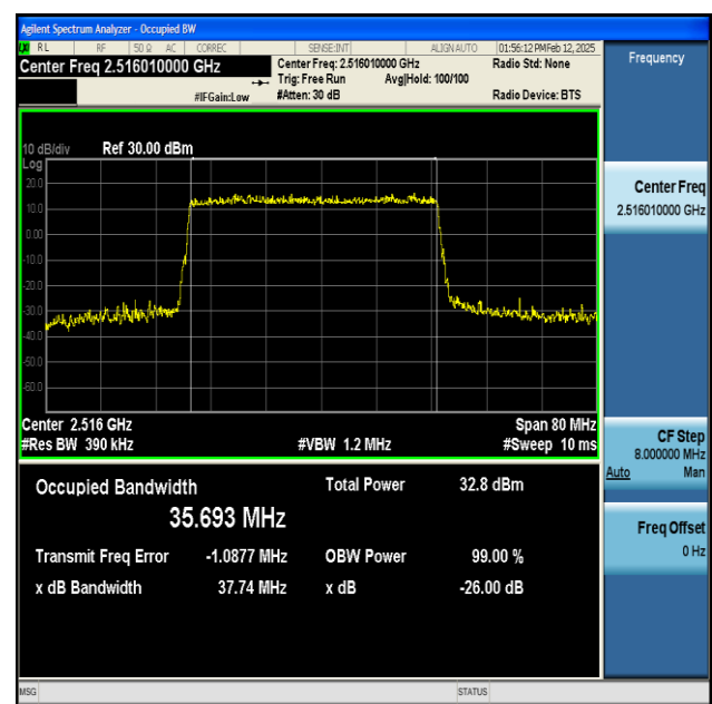
NTNV-n41-PC2-30-40-L-DFT-QPSK-Outer_Full-Ant1- PASS
