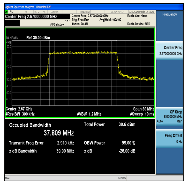
NTNV-n41-PC2-30-40-H-CP-64QAM-Outer_Full-Ant1-PASS
