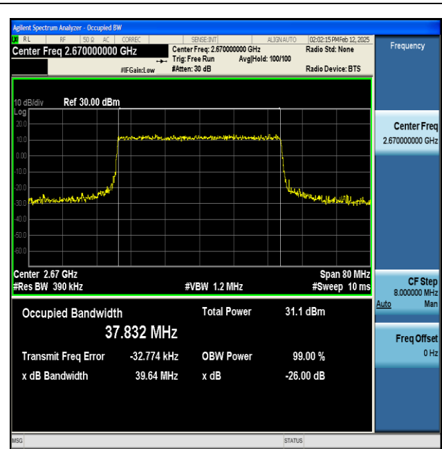
NTNV-n41-PC2-30-40-H-CP-QPSK-Outer_Full-Ant1-PASS
