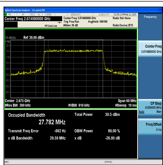
NTNV-n41-PC2-30-30-H-CP-64QAM-Outer_Full-Ant1- PASS
