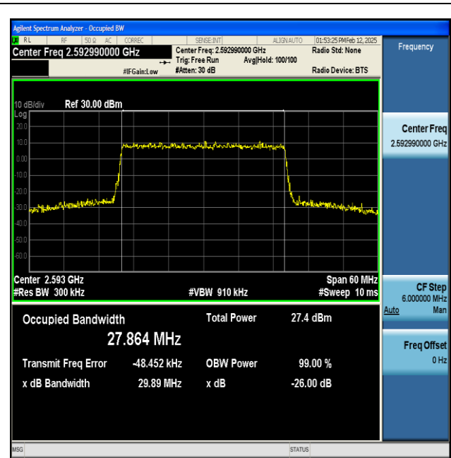
NTNV-n41-PC2-30-30-M-CP-256QAM-Outer_Full-Ant1- PASS
