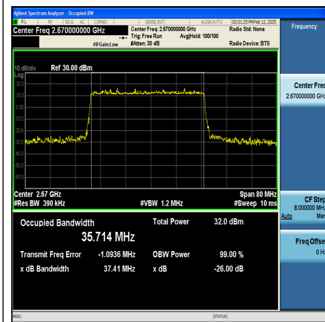
NTNV-n41-PC2-30-40-H-DFT-16QAM-Outer_Full-Ant1- PASS
