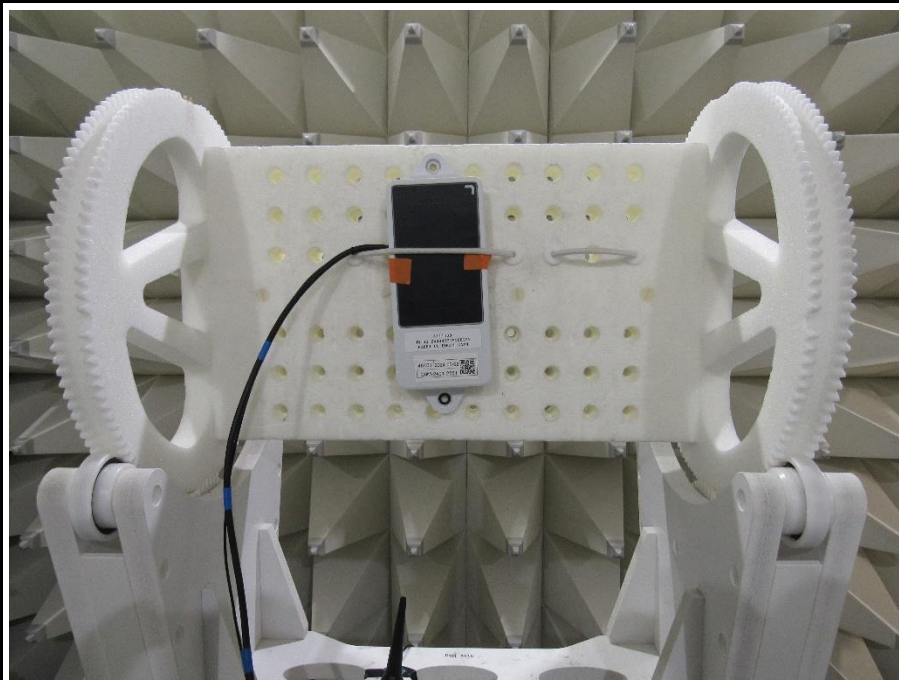
EUT 2 Setup Above 1 GHz
