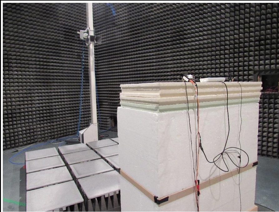
EUT 1 Setup Above 1 GHz
