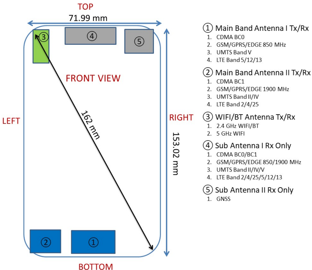
Figure F-1 DUT Antenna Locations
