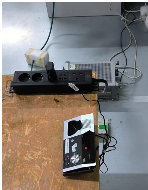
Conducted Emissions - Side View
