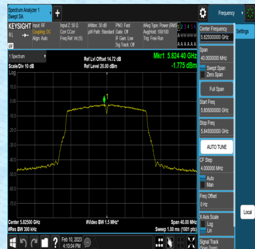
11N20MIMO-Ant1-5825--4.13-0.13-2.22-0.00
