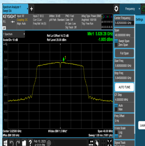
11N20MIMO-Ant2-5825--4.16-0.13-2.22-0.00
