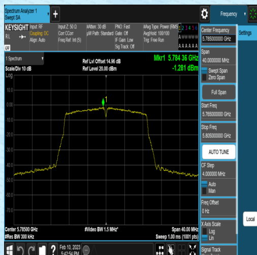
11AC20MIMO-Ant1-5785--3.75-0.25-2.22-0.00
