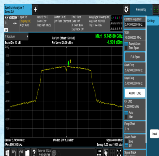
11AC20MIMO-Ant2-5745--4.03-0.31-2.22-0.00
