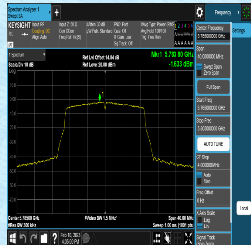
11N20MIMO-Ant1-5785--3.98-0.13-2.22-0.00
