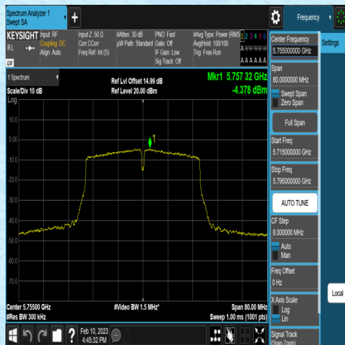
11N40MIMO-Ant1-5755--6.92-0.32-2.22-0.00
