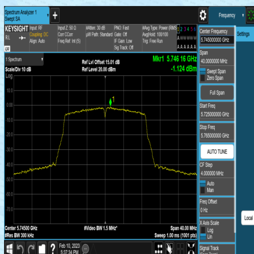
11AC20MIMO-Ant1-5745--3.65-0.31-2.22-0.00
