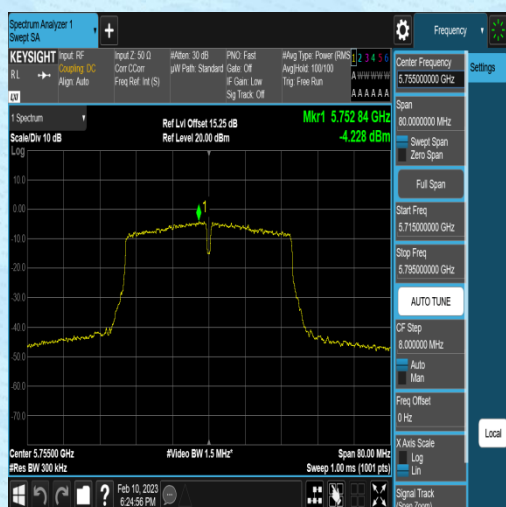
11AC40MIMO-Ant1-5755--7.03-0.58-2.22-0.00
