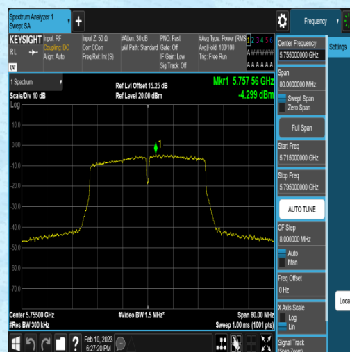
11AC40MIMO-Ant2-5755--7.10-0.58-2.22-0.00
