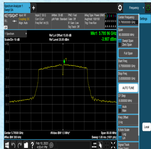
11N40MIMO-Ant2-5795--6.45-0.32-2.22-0.00
