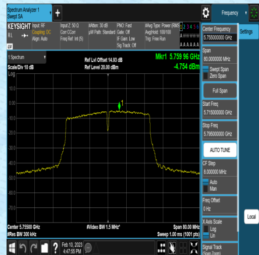
11N40MIMO-Ant2-5755--7.23-0.26-2.22-0.00
