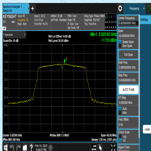
11AC20MIMO-Ant1-5825--4.24-0.31-2.22-0.00
