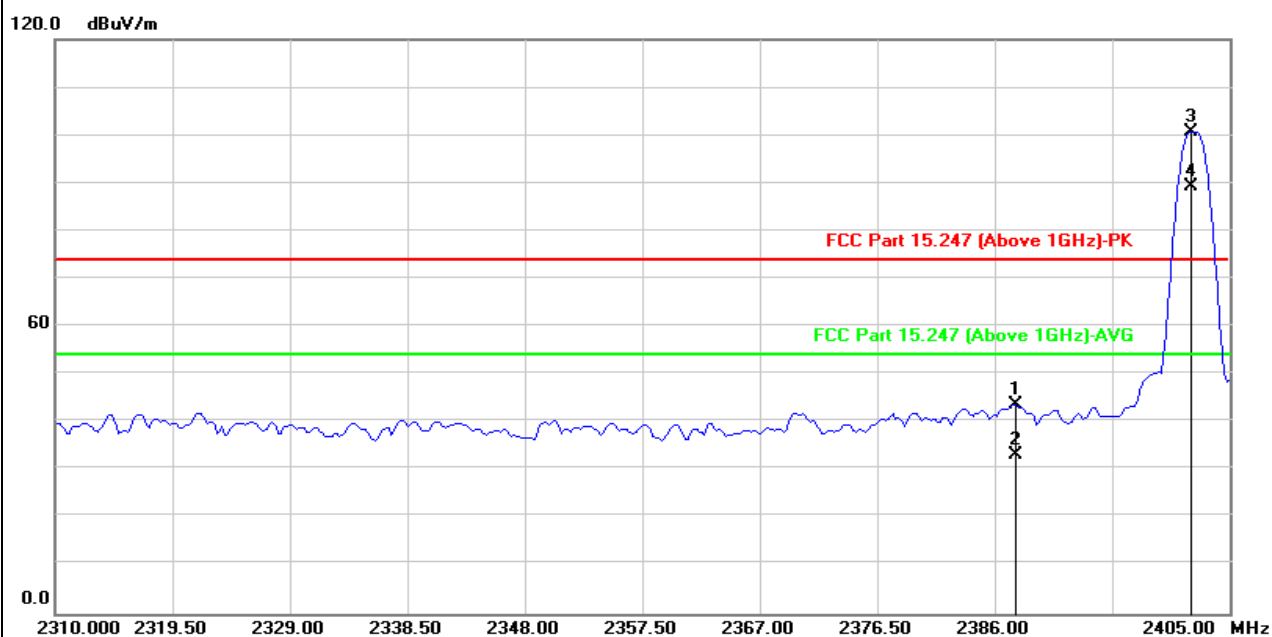
Antennal Polarity&amp; Test Distance: Vertical at 3m
