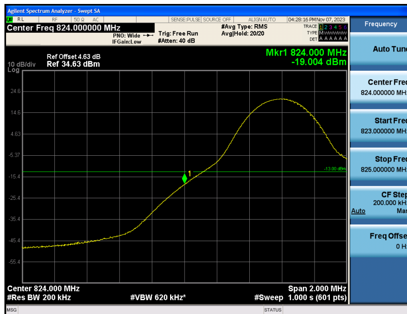
Band5-10MHz-16QAM-20450-1RB#49
